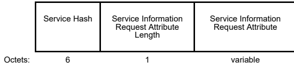
Figure 5: Service Information Request Tuples
