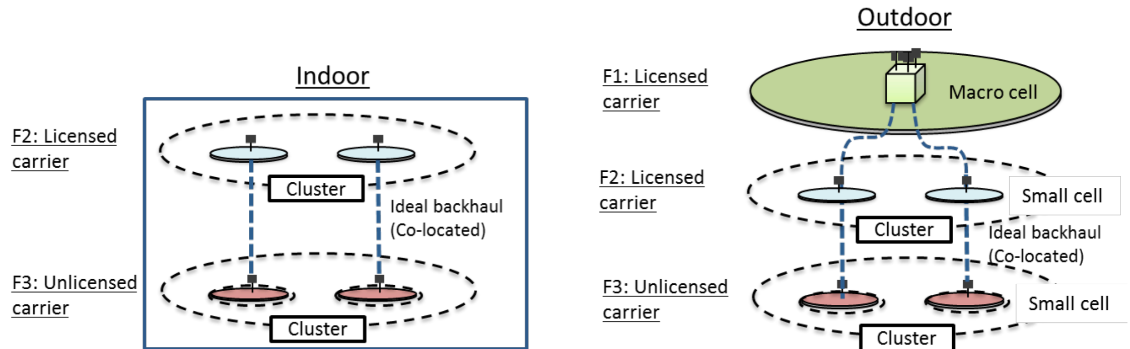
Figure 8.1-1: LAA evaluation scenarios
