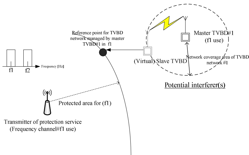
1 2 Figure 20— Example of a reference point on a potential interfering node selection criterion of 3 the interference-victim reference points for the maximum power allocation for multiple 4 TVBDs
