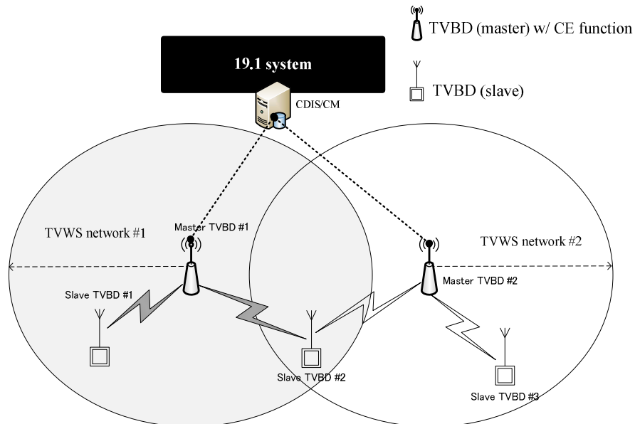
17 18 Figure 14 — Class#2 network geometry
