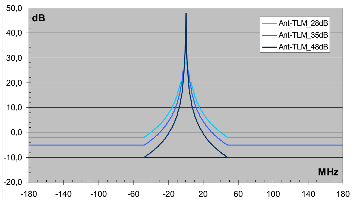
Figure 13: Antenna pattern used for “ground” telemetry stations
