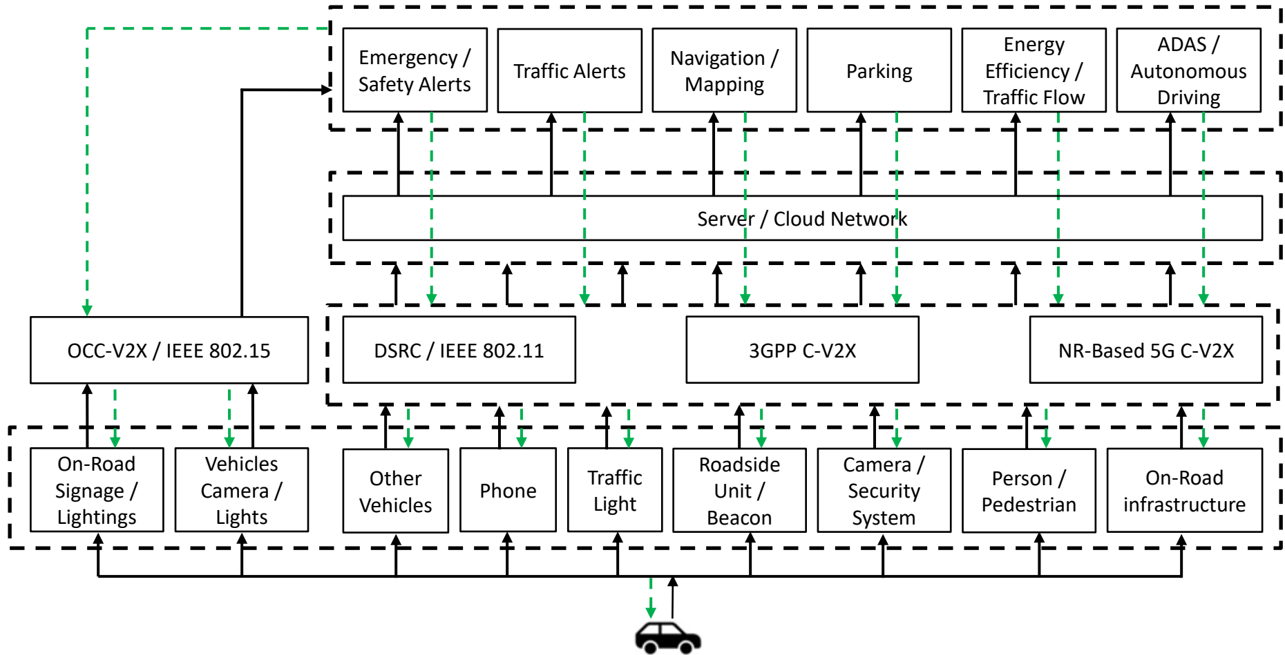
< OCC Enabled V2X Stack Architecture >
