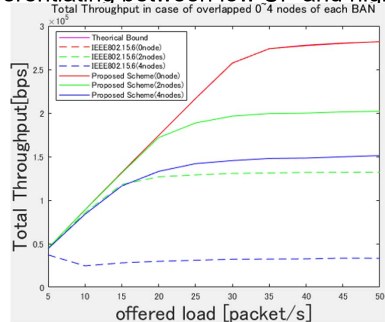
Fig12. Overall network throughput
