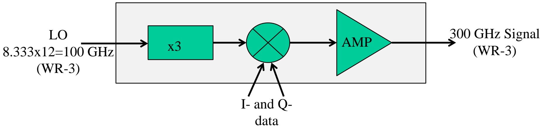
Fully integrated 300 GHz transmitter & receiver MMICs
