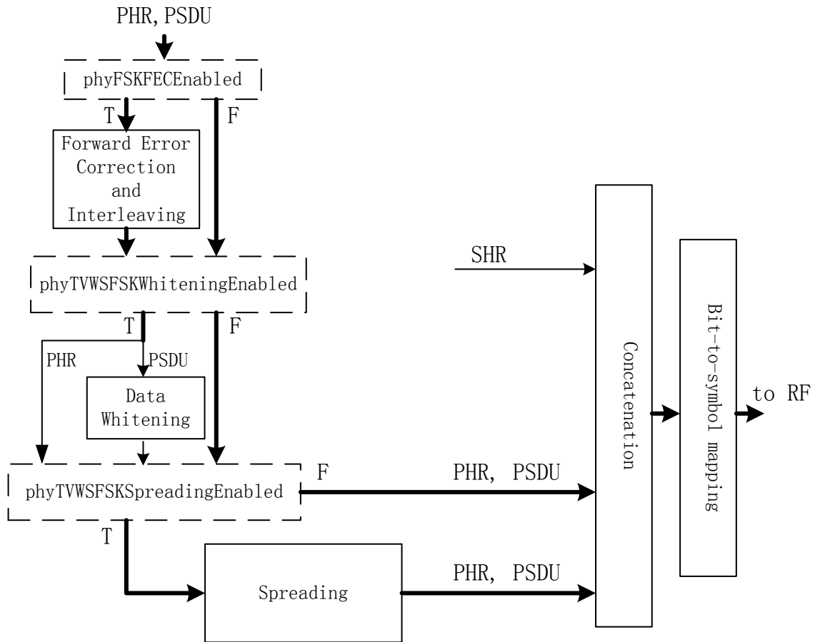
Figure 172—Reference modulator diagram for TVWS-FSK
