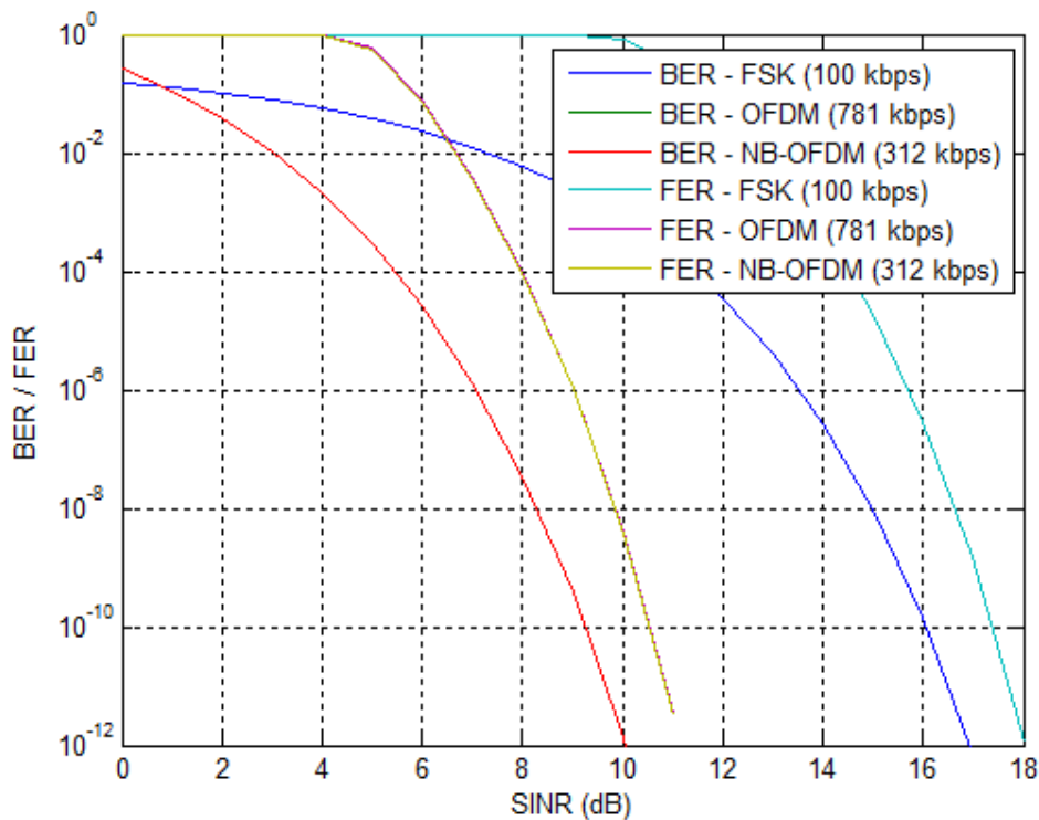
Figure 7: BER/FER vs. SINR for 802.15.4m PHYs
