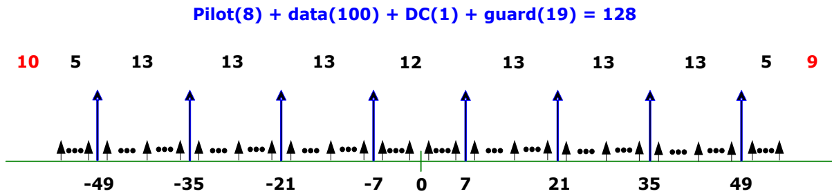
Figure 135 - Pilot tones for TVWS OFDM
