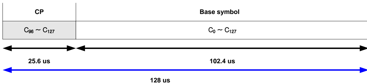
Figure 136-Cyclic prefix (CP)
