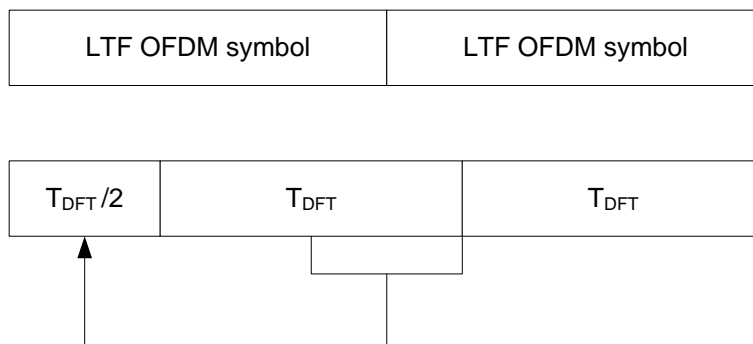
Figure 130-Structure of LTF for TVWS-OFDM
