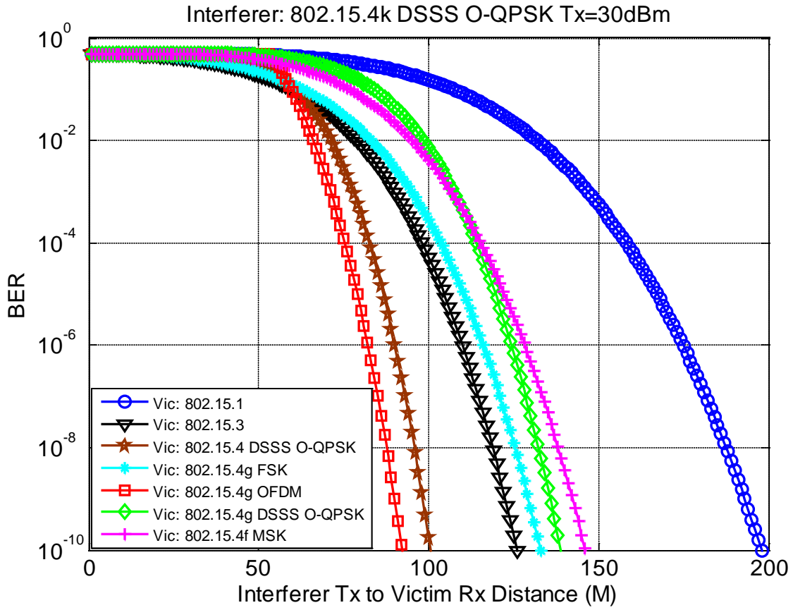
Figure 47: Victim BER vs. Distance from Interferer Tx (30dm) to 802.15 Victim Rx
