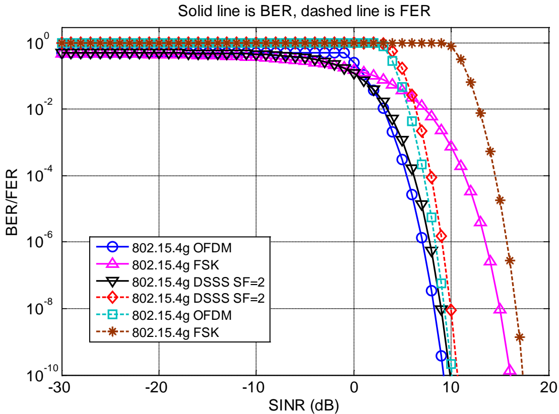
Figure 11: BER and FER vs. SINR for 802.15.4g Systems (470 - 510MHz band)
