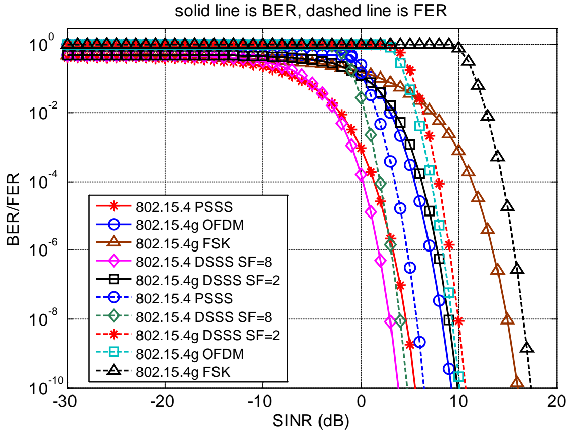
Figure 24: BER and FER vs. SINR for 802.15.4 & 4g Systems (863 - 870MHz band)
