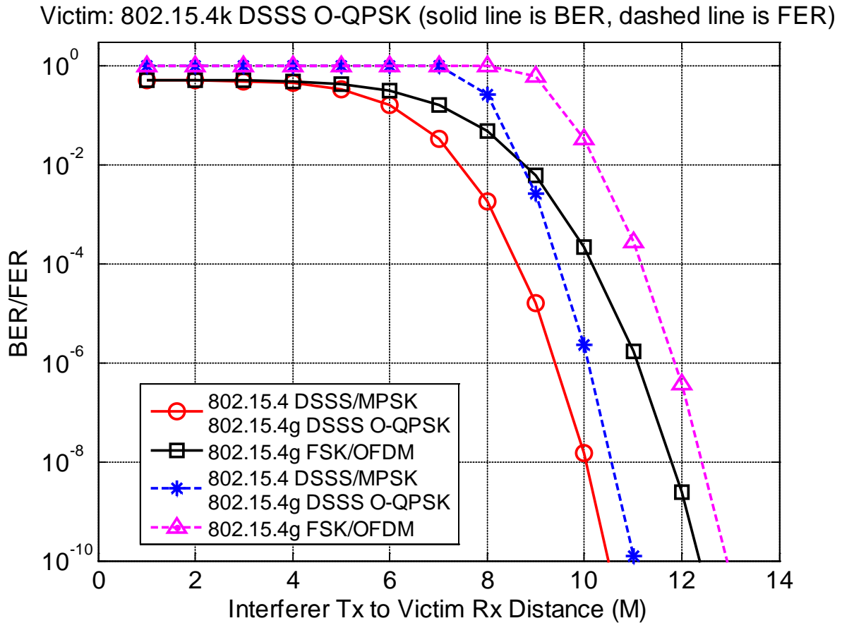
Figure 19: Victim BER/FER vs. Distance from Interferer Tx to 802.15.4k DSSS Victim Rx
