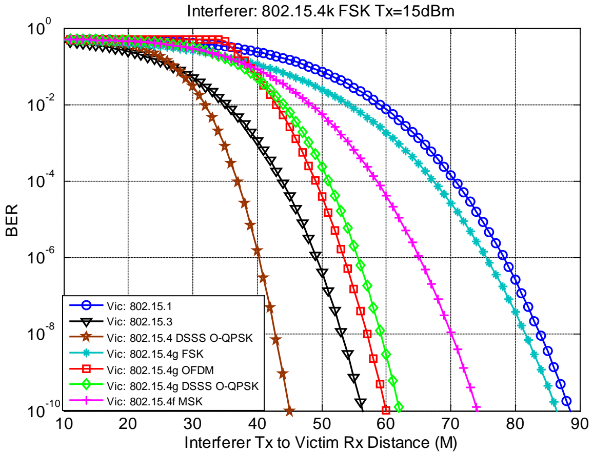
Figure 52: Victim BER vs. Distance from Interferer Tx (15dBm) to 802.15 Victim Rx
