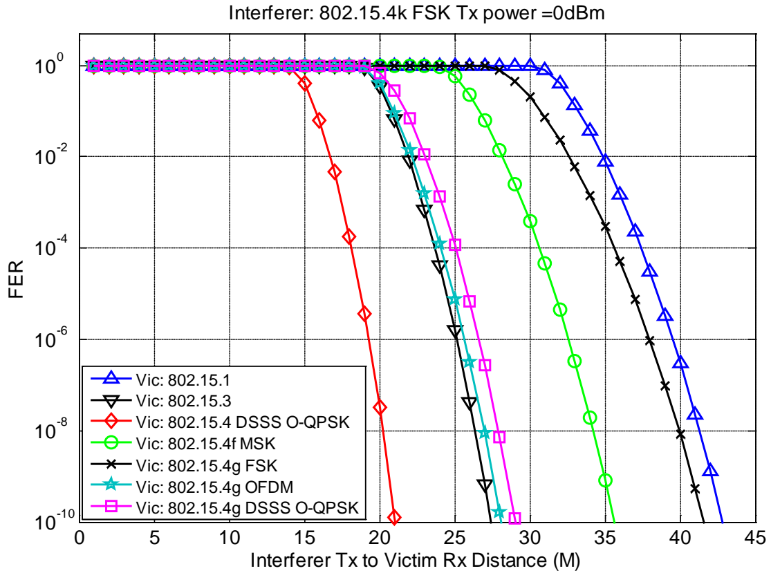
Figure 54: Victim FER vs. Distance from Interferer Tx (0dBm) to 802.15 Victim Rx
