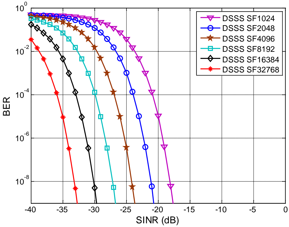
Figure 2: BER vs. SINR for 802.15.4k DSSS (2.4GHz band)
