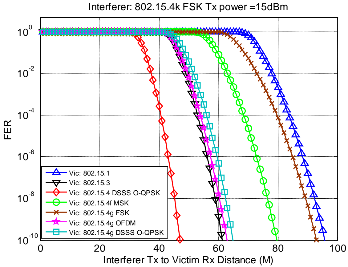
Figure 55: Victim FER vs. Distance from Interferer Tx (15dBm) to 802.15 Victim Rx
