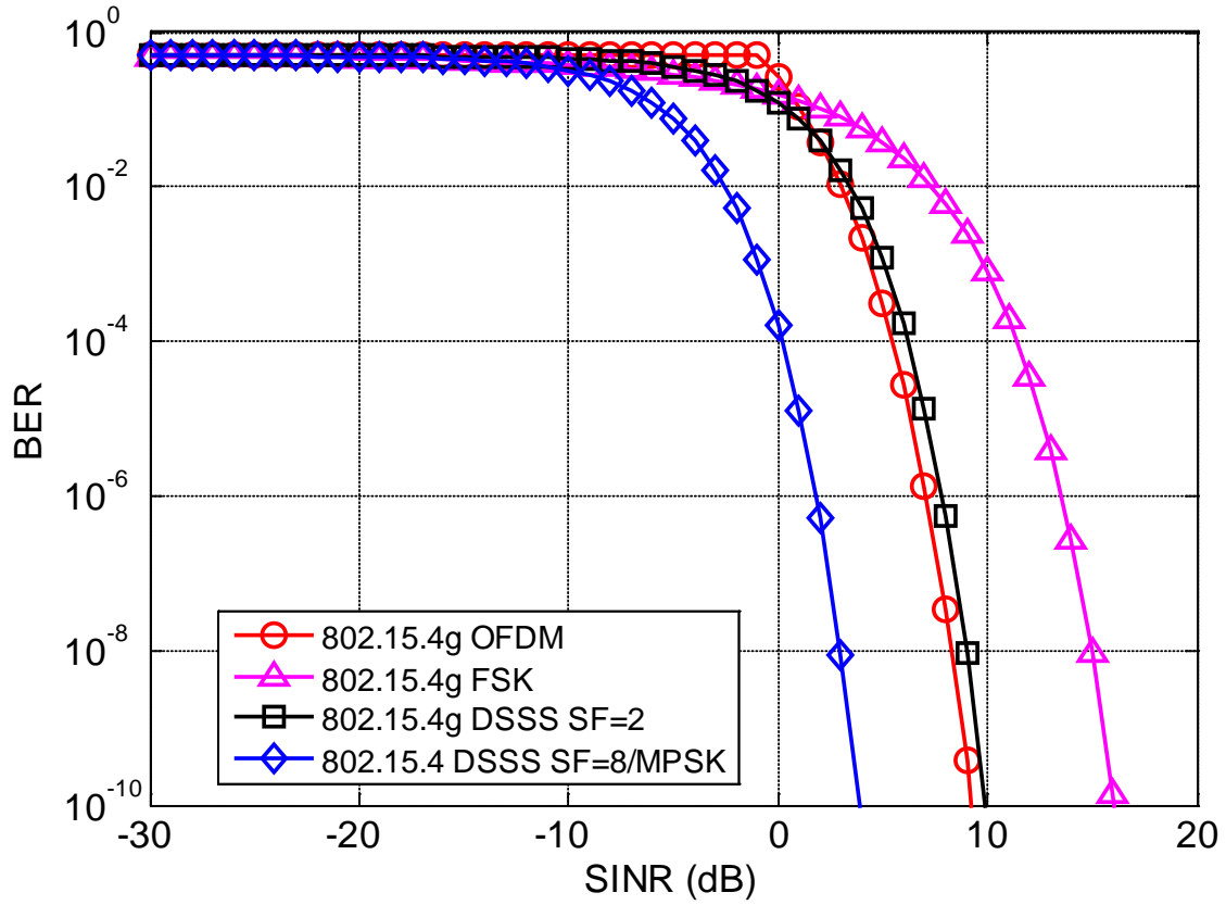
Figure 17: BER vs. SINR for 802.15.4 & 4g Systems (779 – 787MHz band)
