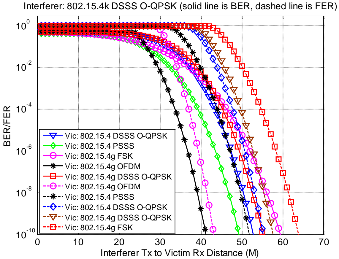
Figure 28: Victim BER/FER vs. Distance from Interferer Tx to 802.15.4 and 802.15.4g Victim Rx
