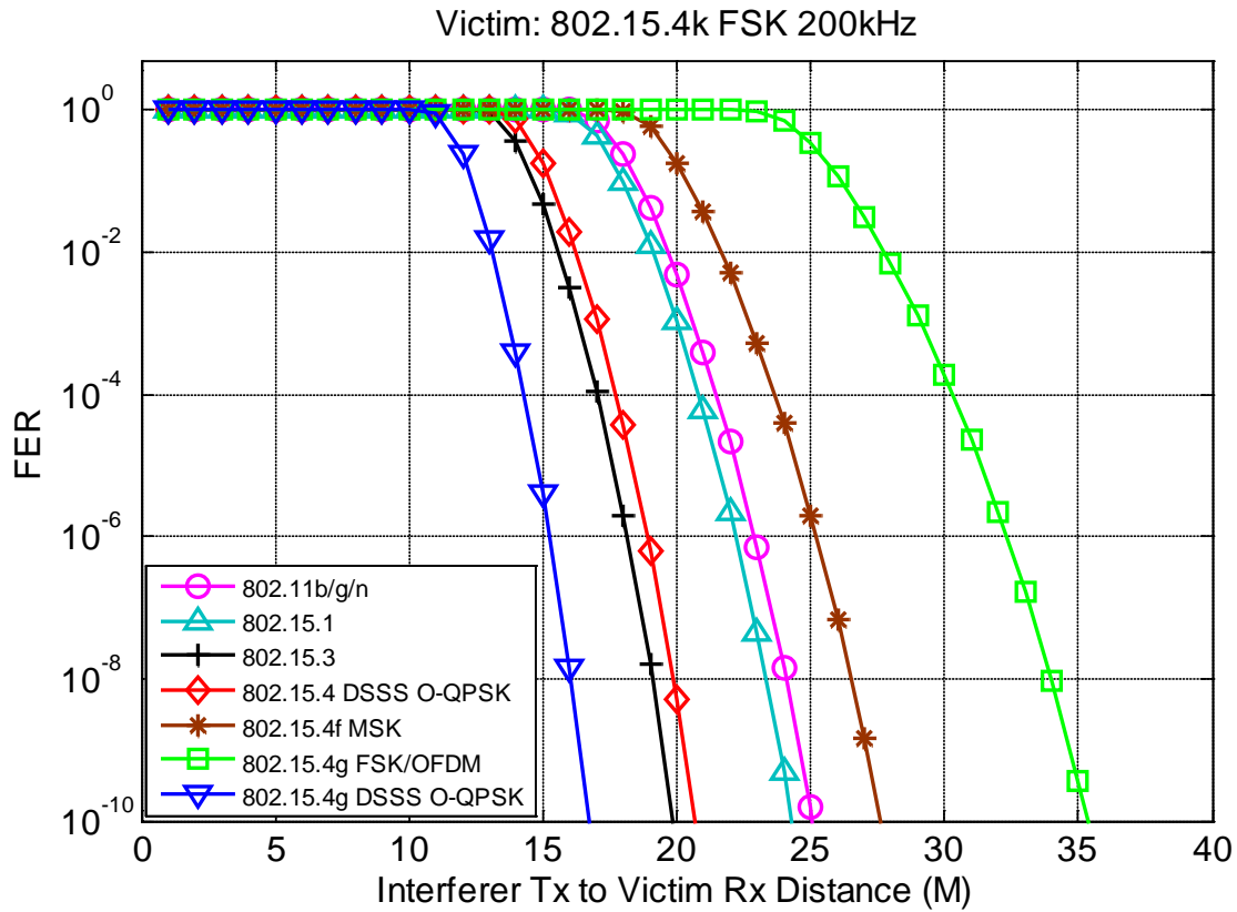
Figure 41: Victim FER vs. Distance from Interferer Tx to 802.15.4k FSK Victim Rx (200 kHz)
