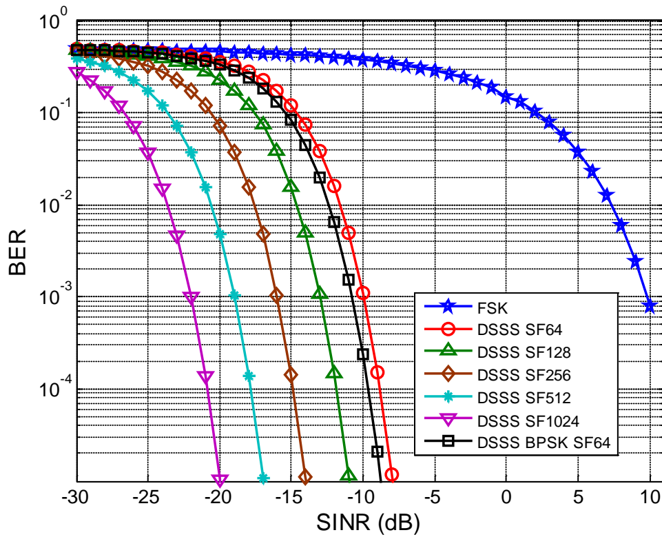
Figure 1: BER vs. SINR for 802.15.4k FSK and DSSS (2.4GHz band)
