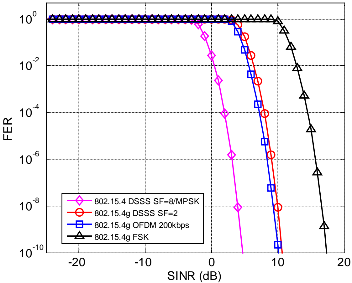
Figure 18: FER vs. SINR for 802.15.4 & 4g Systems (779 – 787MHz band)
