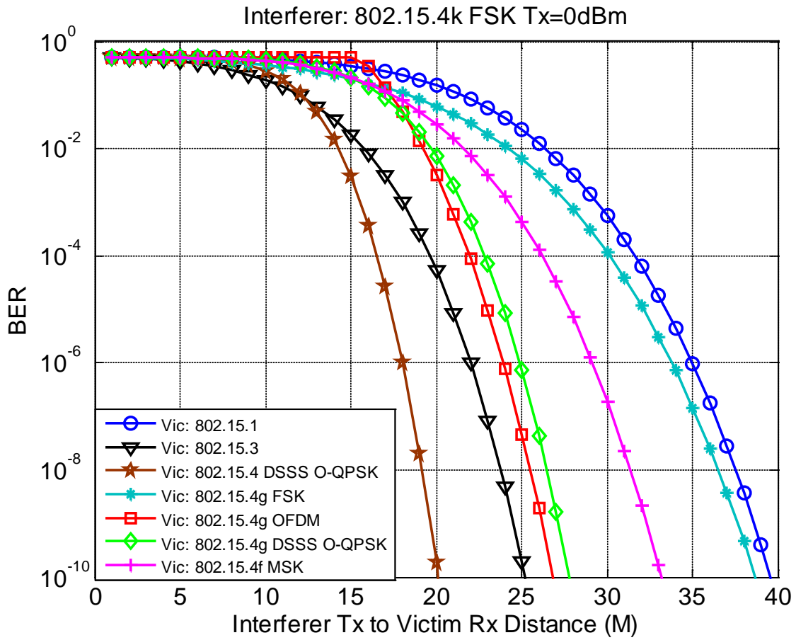
Figure 51: Victim BER vs. Distance from Interferer Tx (0dBm) to 802.15 Victim Rx
