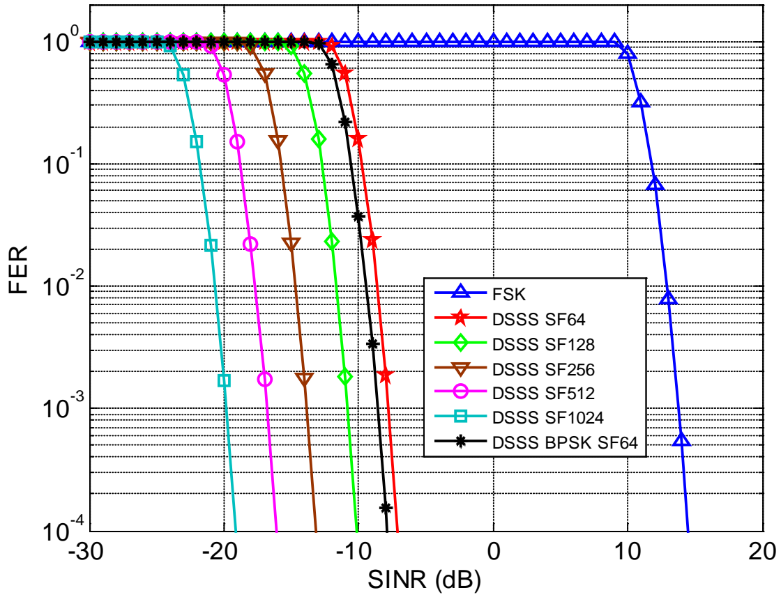
Figure 3: FER vs. SINR for 802.15.4k FSK and DSSS (2.4GHz band)
