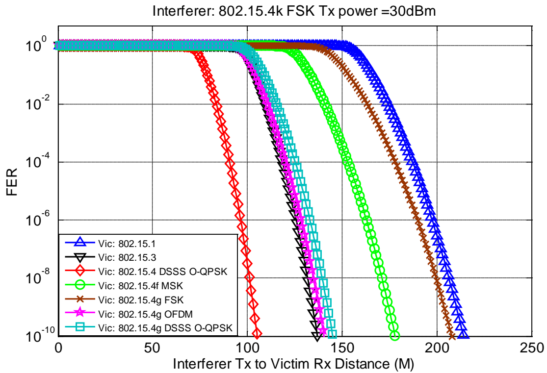
Figure 56: Victim FER vs. Distance from Interferer Tx (30dBm) to 802.15 Victim Rx
