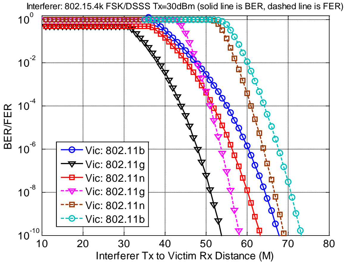
Figure 44: Victim BER/FER vs. Distance from Interferer Tx (30dBm) to 802. 11 Victim Rx
