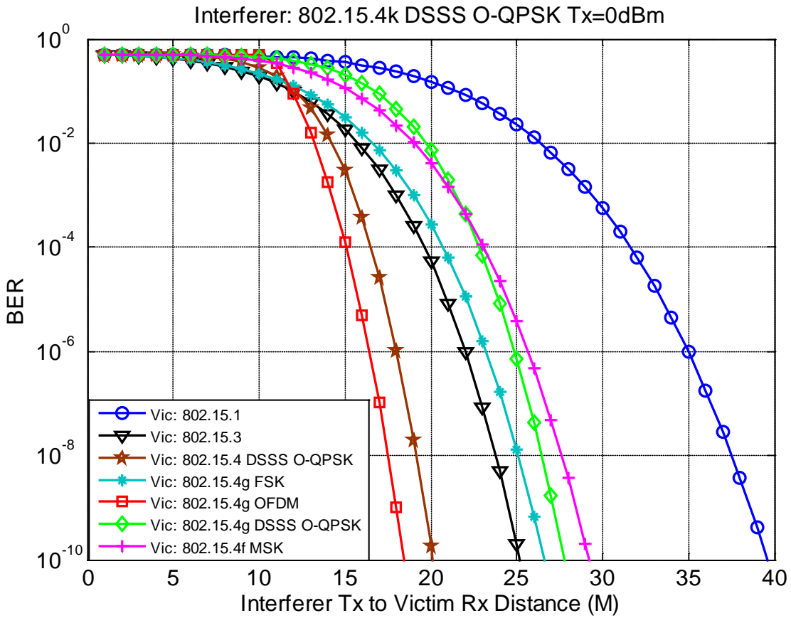
Figure 45: Victim BER vs. Distance from Interferer Tx (0dBm) to 802.15 Victim Rx
