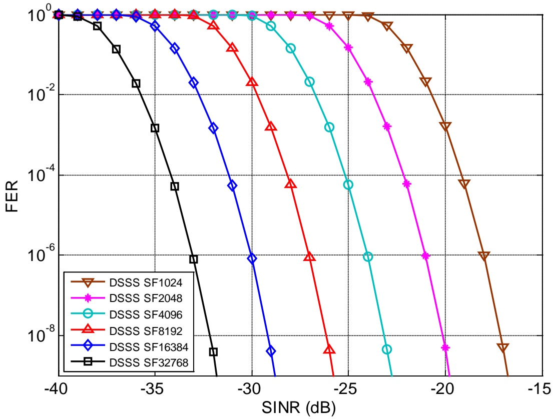
Figure 4: FER vs. SINR for 802.15.4k DSSS (2.4GHz band)
