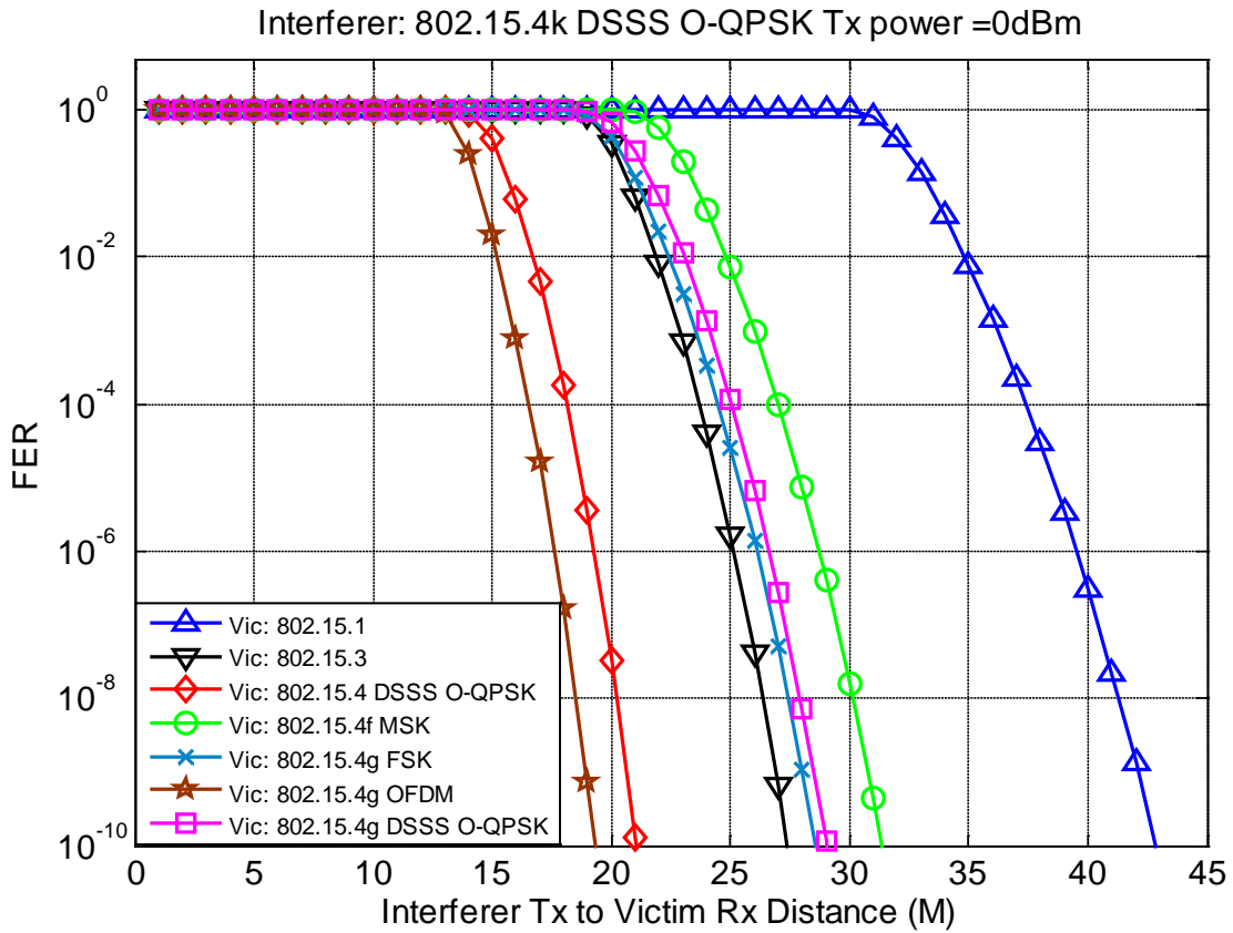
Figure 48: Victim FER vs. Distance from Interferer Tx (0dBm) to 802.15 Victim Rx
