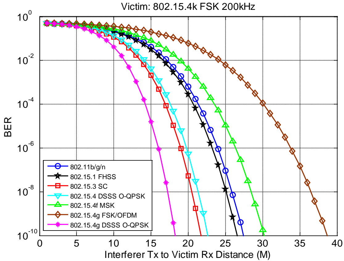
Figure 40: Victim BER vs. Distance from Interferer Tx to 802.15.4k FSK Victim Rx (200 kHz)
