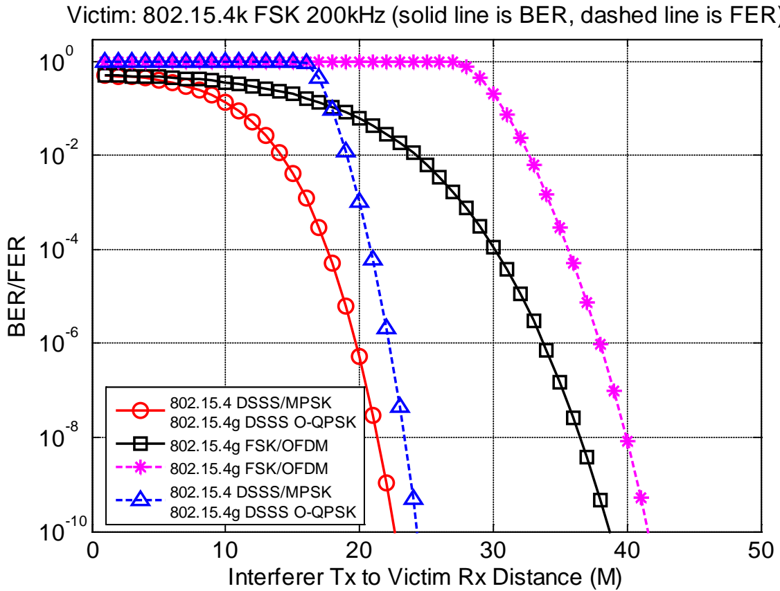
Figure 21: Victim BER/FER vs. Distance from Interferer Tx to 802.15.4k FSK Victim Rx (200 kHz)
