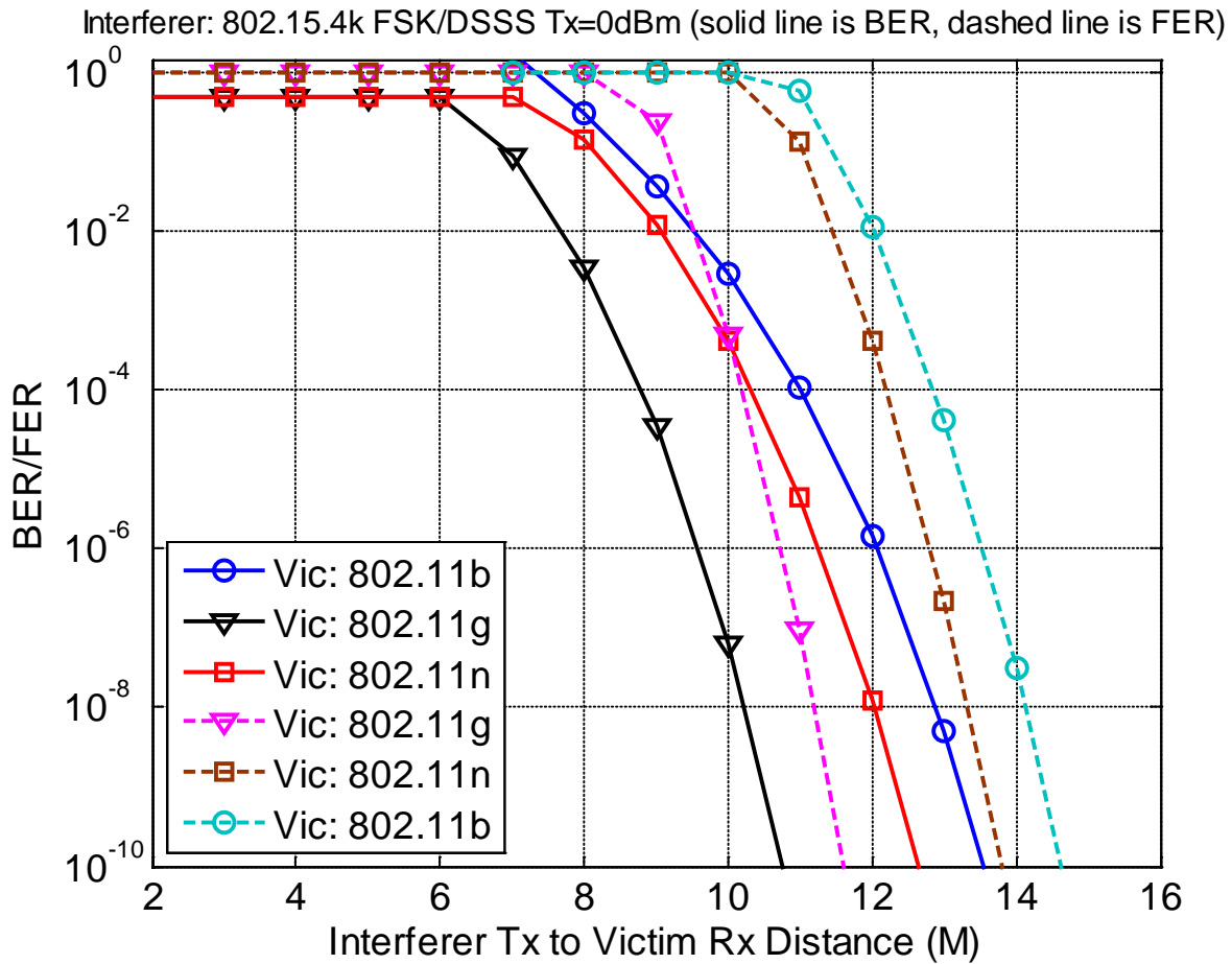
Figure 42: Victim BER/FER vs. Distance from Interferer Tx (0dBm) to 802.11 Victim Rx
