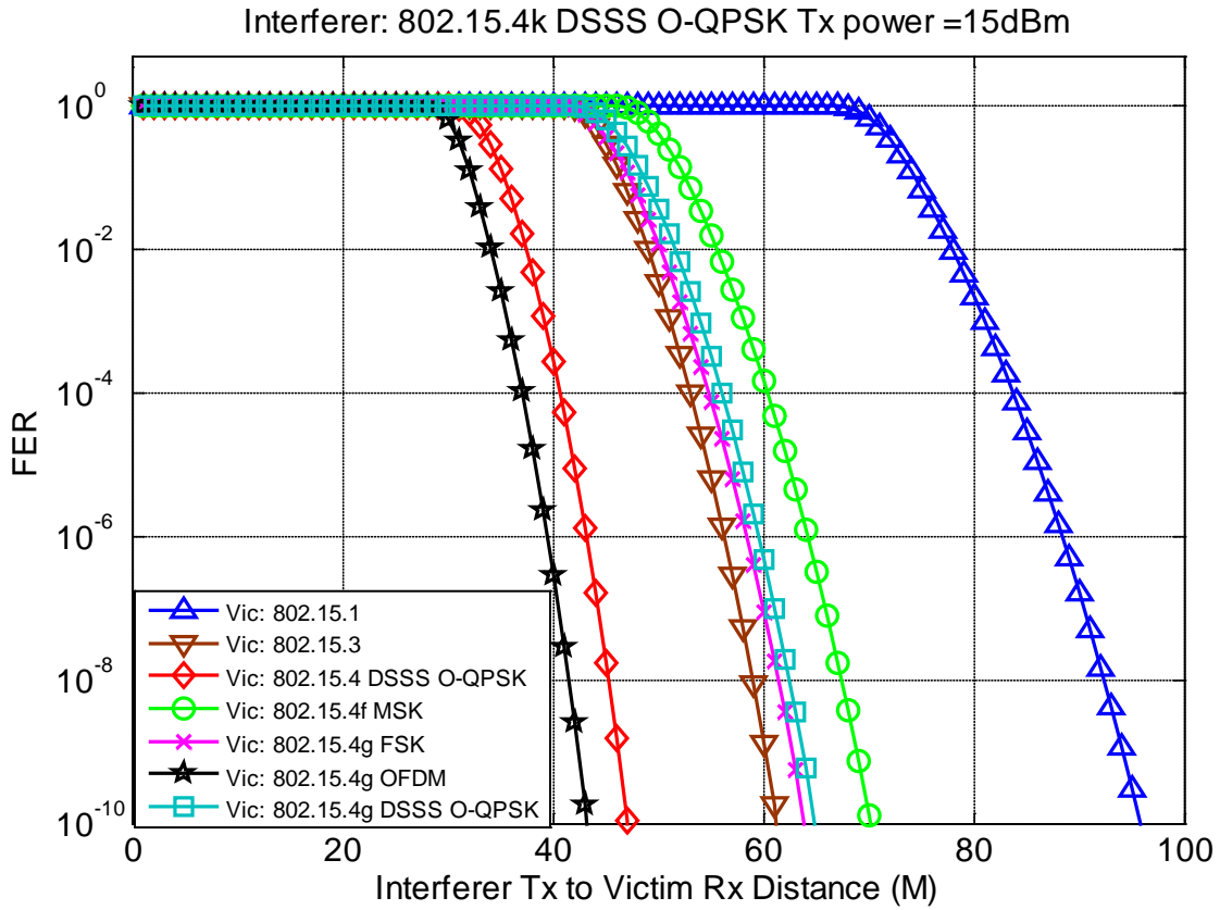
Figure 49: Victim FER vs. Distance from Interferer Tx (15dBm) to 802.15 Victim Rx
