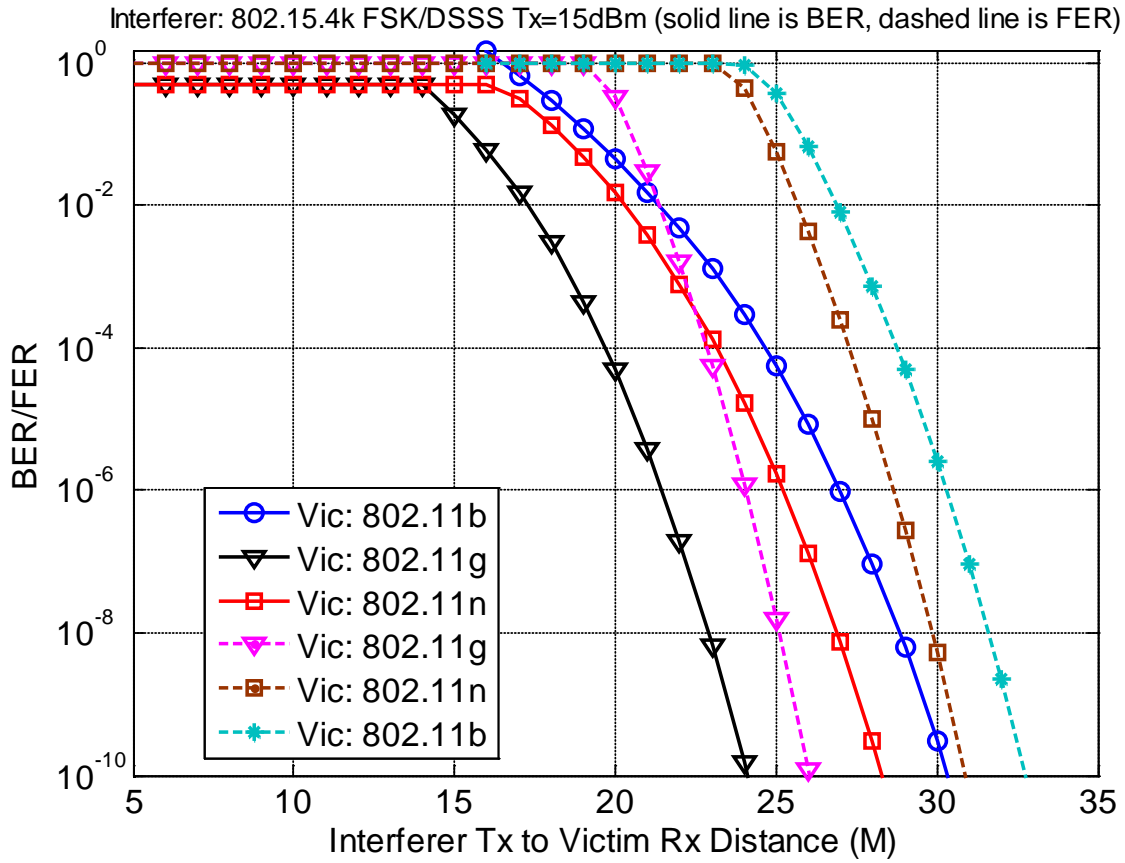
Figure 43: Victim BER/FER vs. Distance from Interferer Tx (15dBm) to 802. 11 Victim Rx
