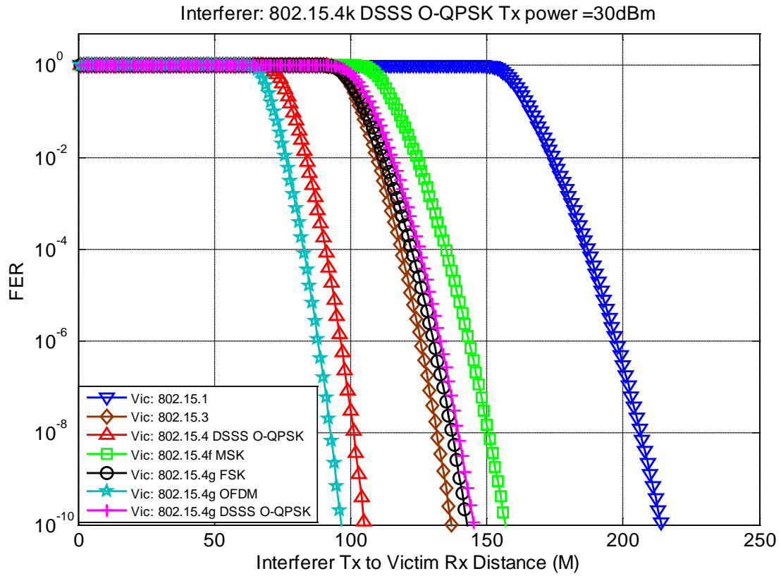
Figure 50: Victim FER vs. Distance from Interferer Tx (30dBm) to 802.15 Victim Rx
