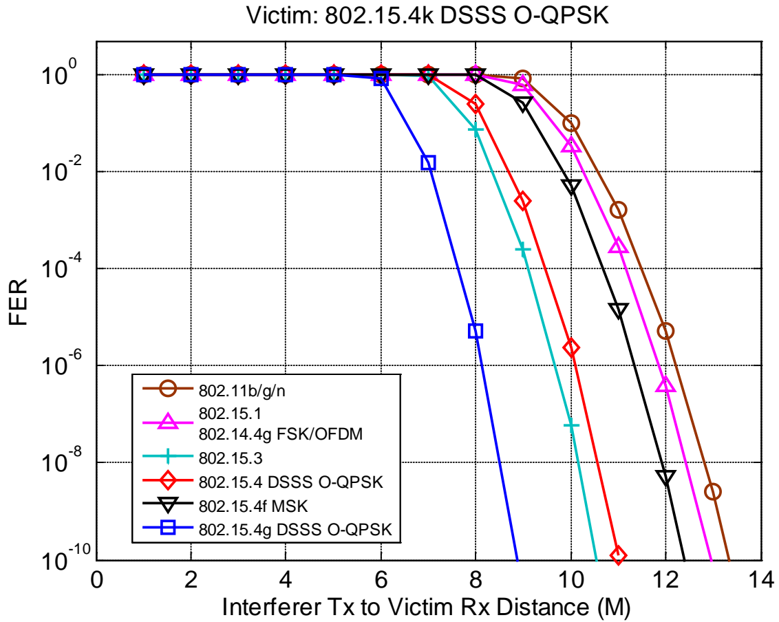
Figure 39: Victim FER vs. Distance from Interferer Tx to 802.15.4k DSSS Victim Rx
