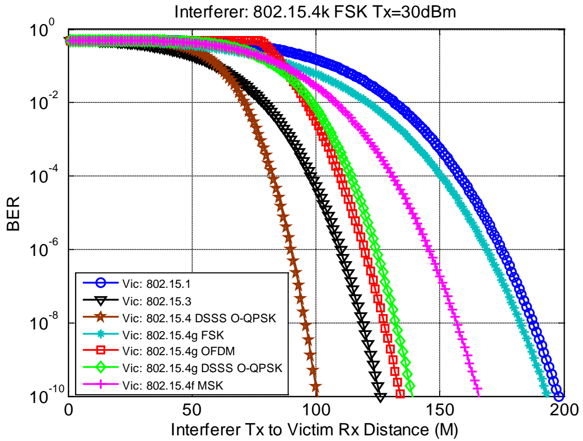
Figure 53: Victim BER vs. Distance from Interferer Tx (30dBm) to 802.15 Victim Rx
