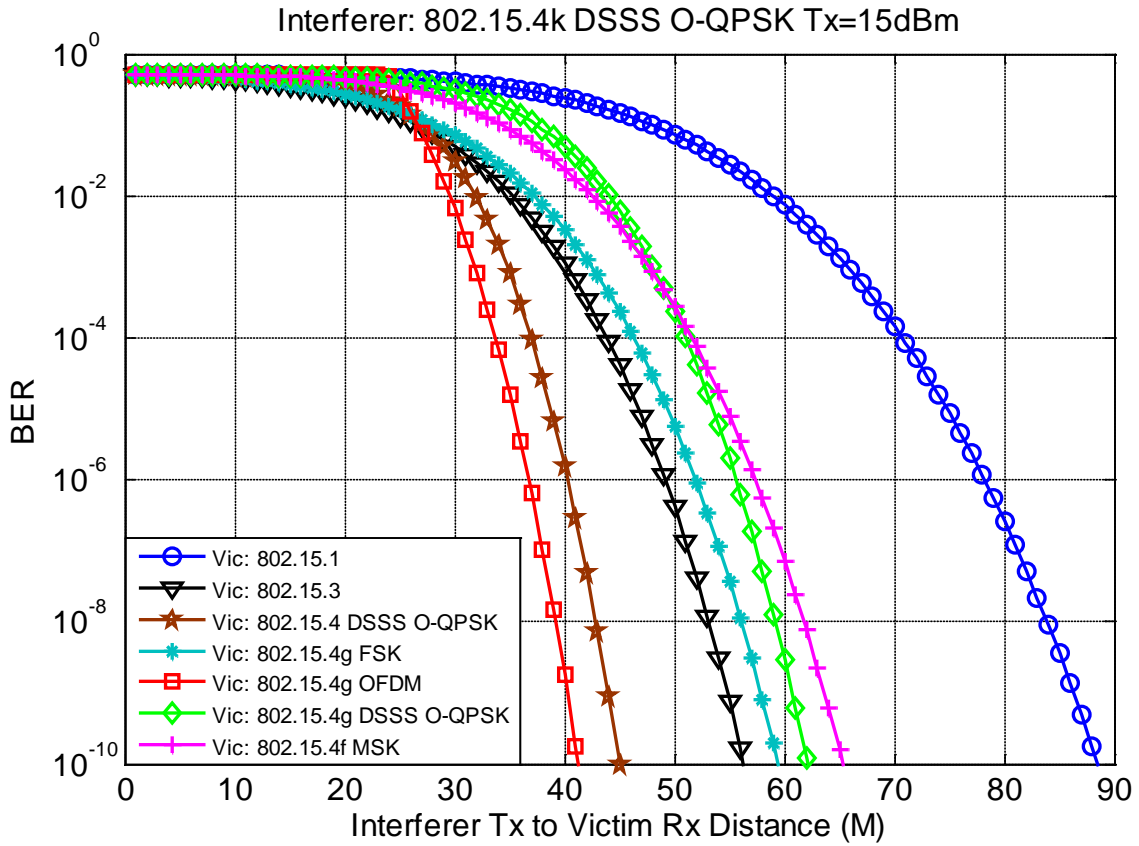
Figure 46: Victim BER vs. Distance from Interferer Tx (15dBm) to 802.15 Victim Rx
