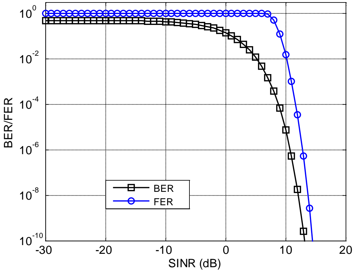
Figure 8: BER/FER vs. SINR for 802.15.4f (433.05 – 434.79MHz band)
