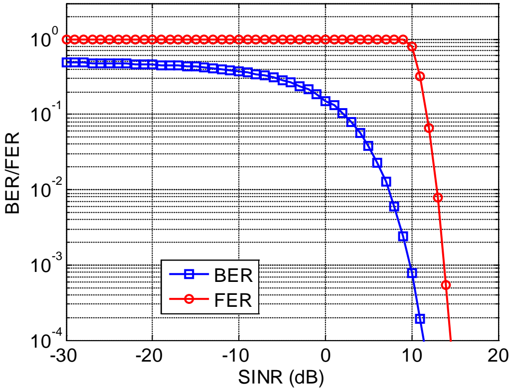
Figure 5: BER/FER vs. SINR for 802.15.4g MR-FSK (169.400 - 169.475MHz band)
