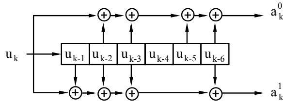
Figure 70—Convolutional encoder
