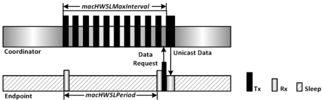
Figure 34sc—Unicast transmission in HWSL mode
