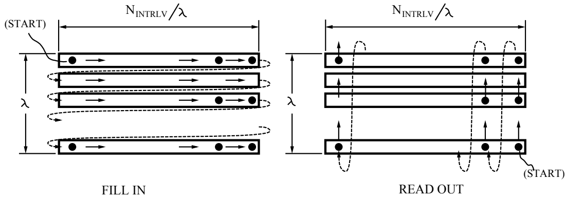
Figure 72—Interleaver
