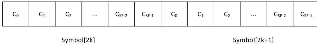
Figure 64—BPSK chip modulation
