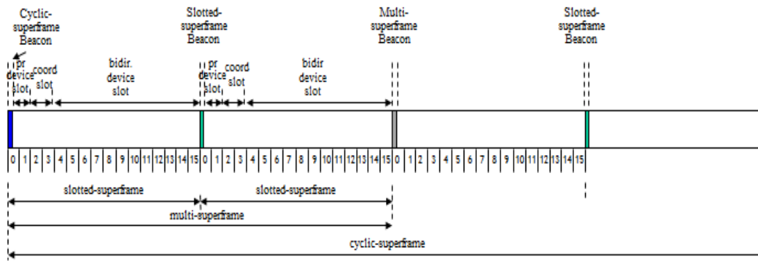
Figure 4c—An example of the cyclic-superframe structure
