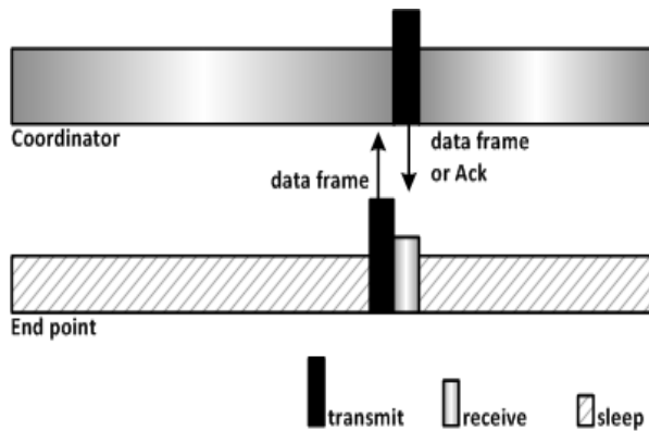
Figure 34sb—Basic LECIM LE mode operations
