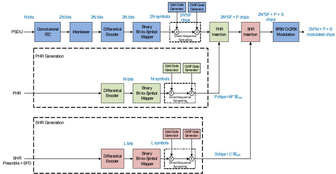
Figure 61—LECIM DSSS reference modulator diagram
