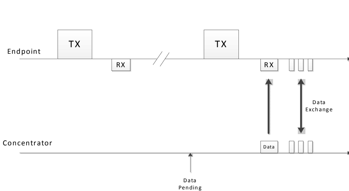
Figure 34se—I-RIT transmission
