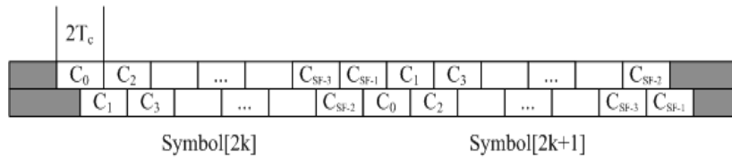
Figure 65—O-QPSK chip modulation
