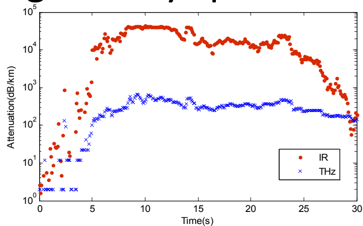
Specific attenuation of THz link and IR link over time
