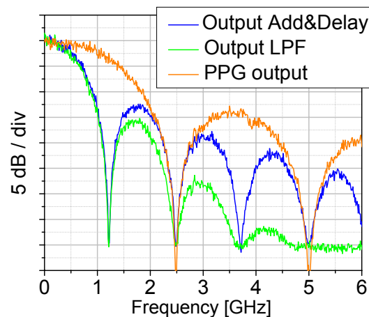
Spectra of baseband signals
