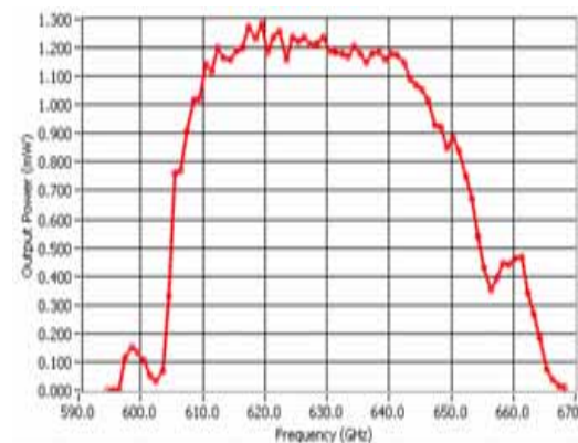
50 GHz source tuning range.
