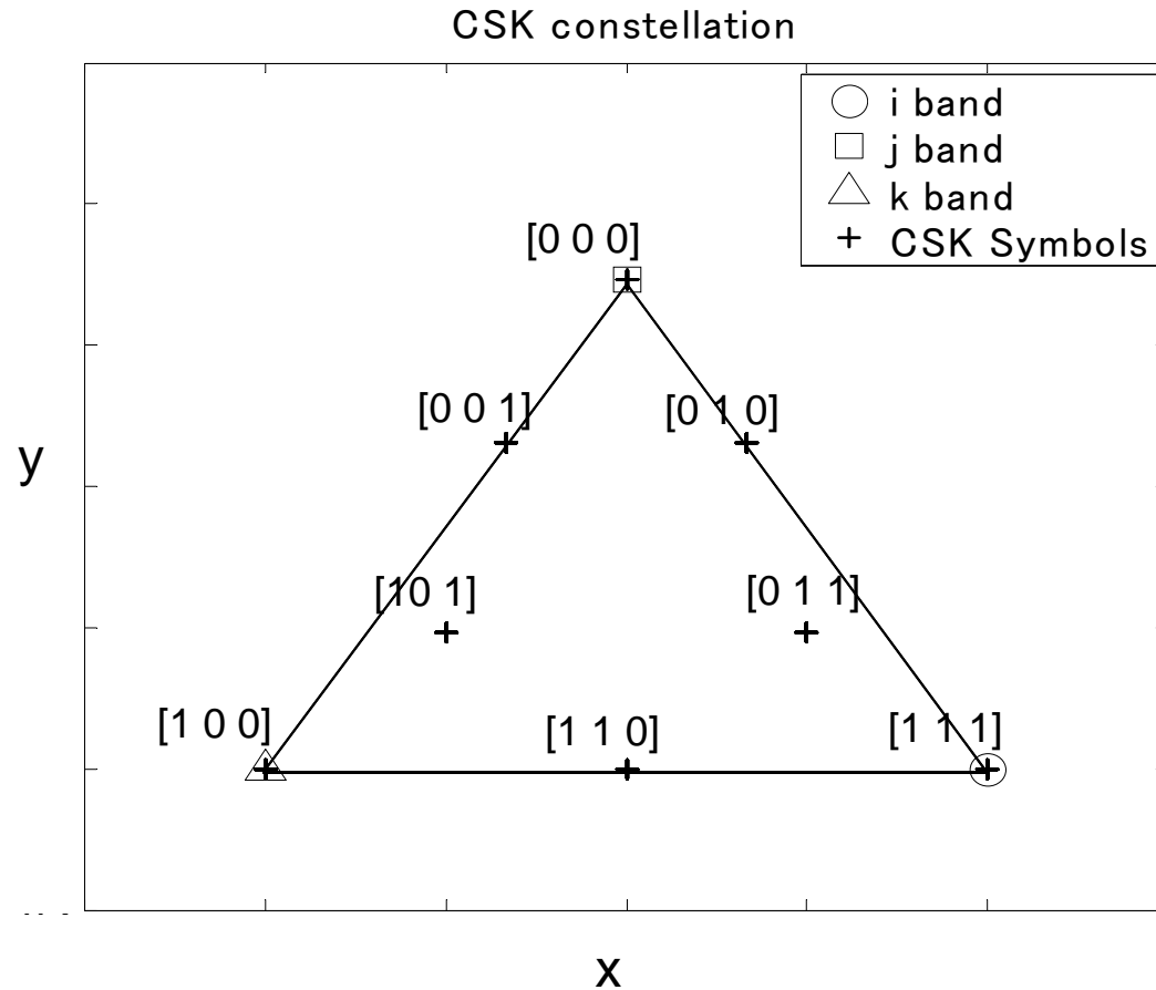
Fig.141 - Data mapping for 8-CSK
