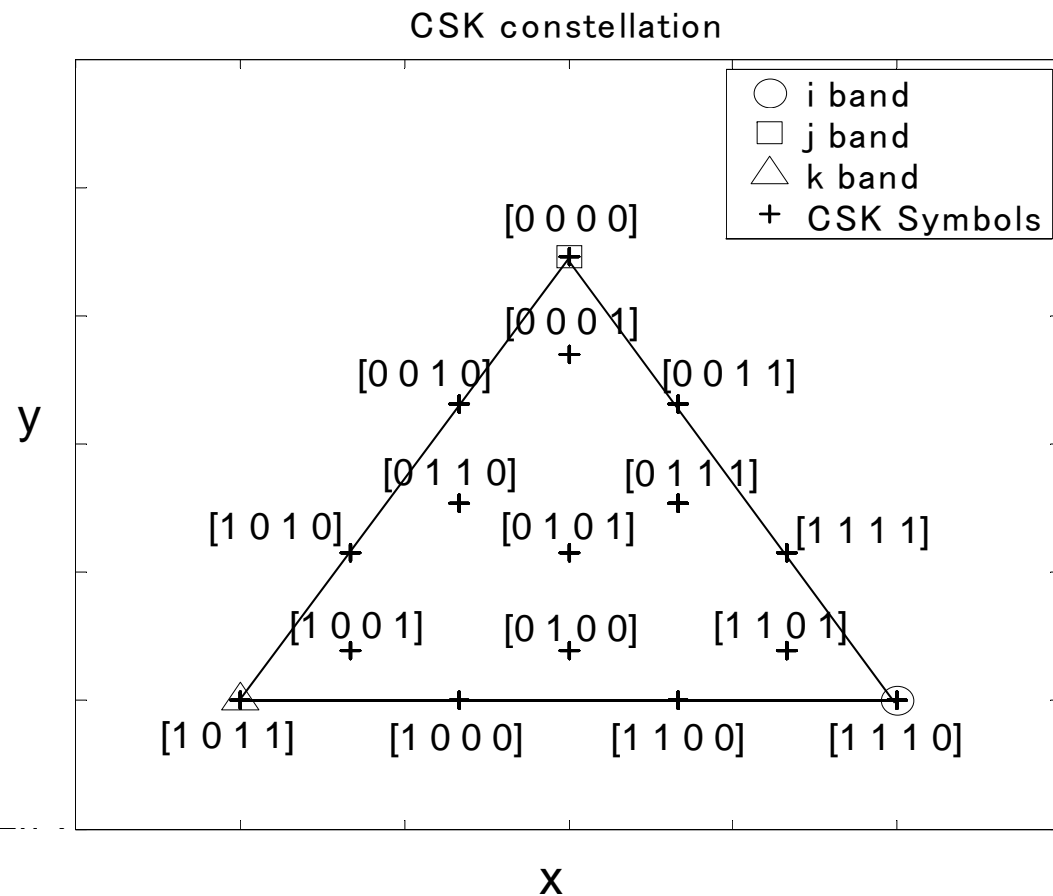
Fig.142 - Data mapping for 16-CSK
