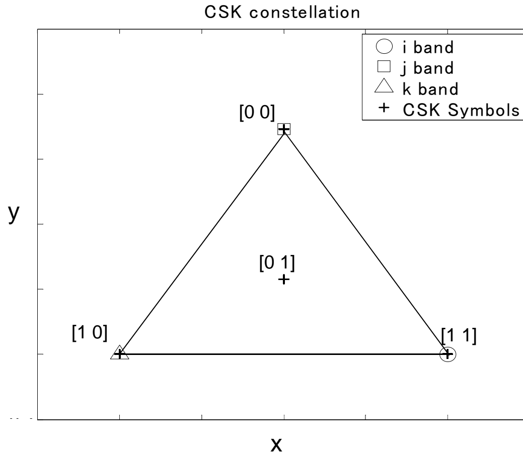
Fig.140 - Data mapping for 4-CSK
