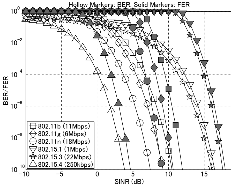
Figure 3 BER/FER vs. SINR for 802 Systems in the 2400-2483.5 MHz Band
