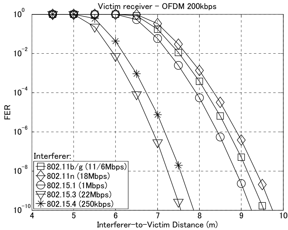
Figure 5 FER vs. Distance between Interferer to 802.15.4g OFDM Victim Receiver
