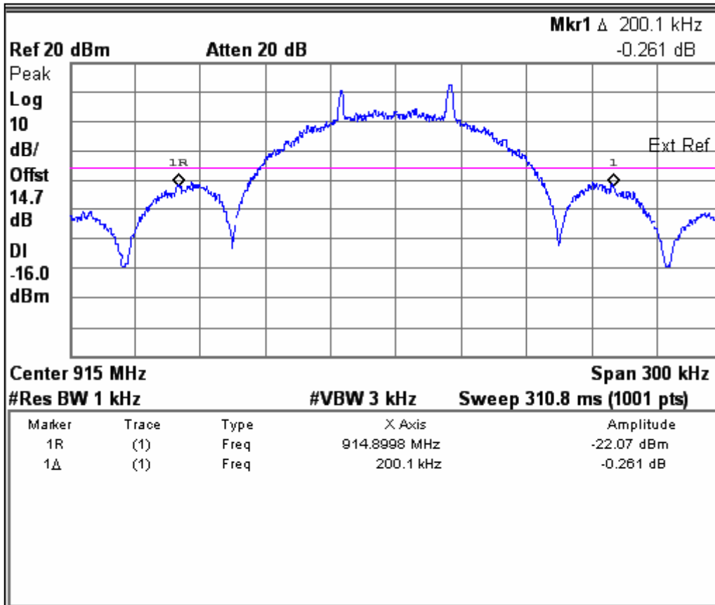
Figure 2: Measurement of Modulation Bandwidth to ETSI EN 300 220-1
