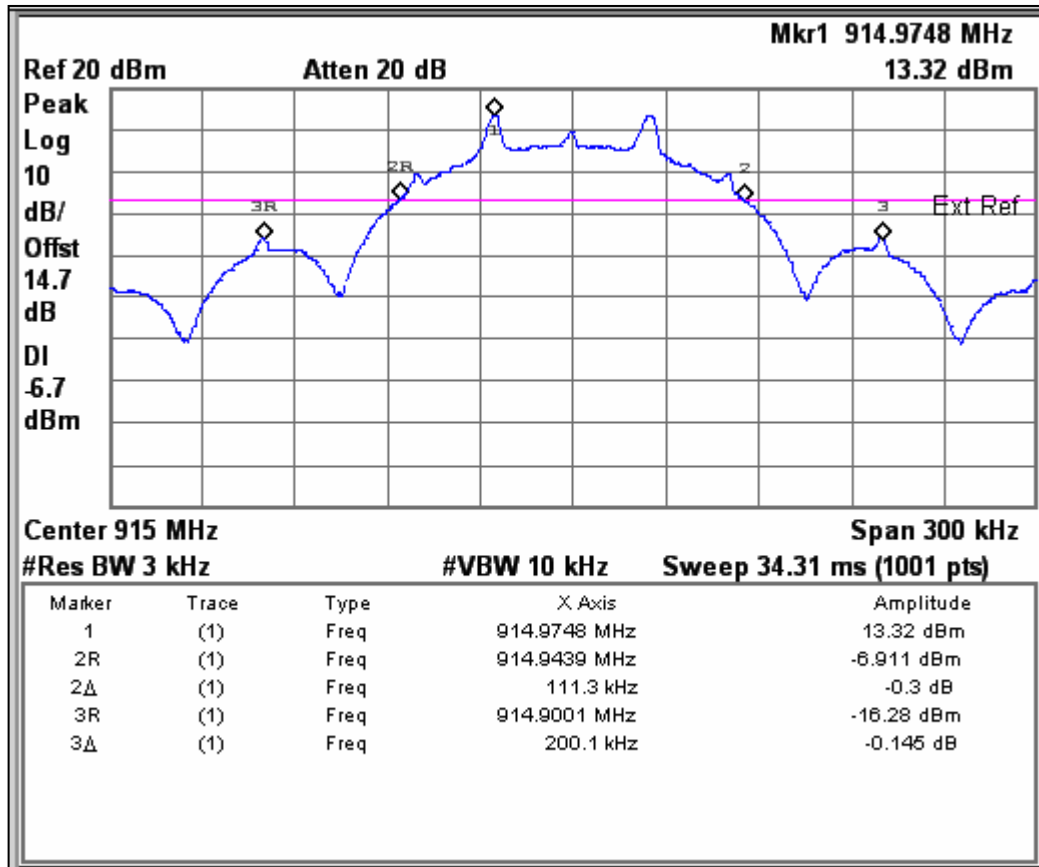
Figure 1: Measurement of Adjacent Channel Attenuation to FCC DA 00-705
