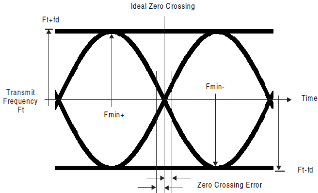
Figure 1—Modulation figure for 802.15.1
