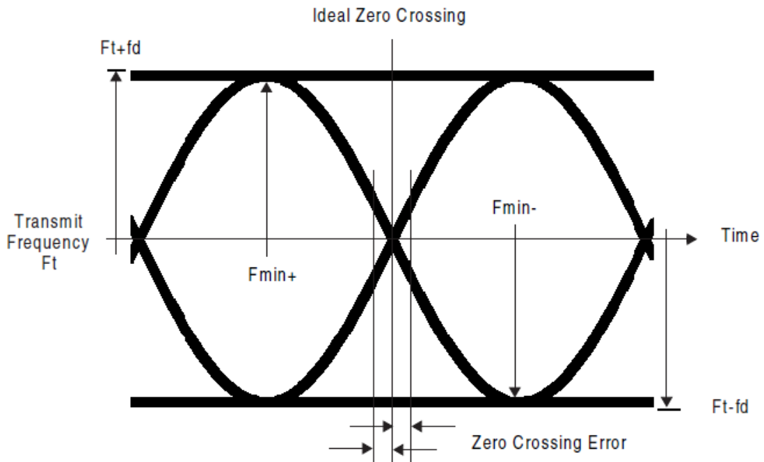
Figure 2—2-FSK modulation
