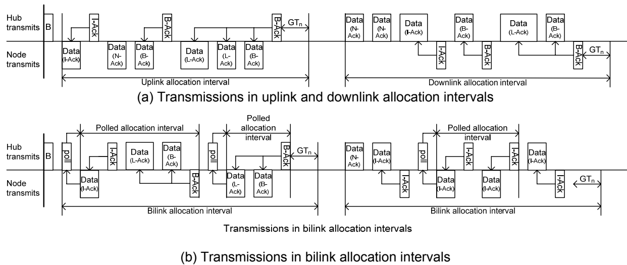
Figure 40 — Example frame transactions in scheduled allocation intervals
