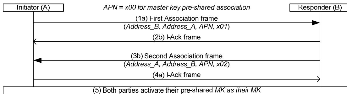
Figure 63 — MK pre-shared association procedure
