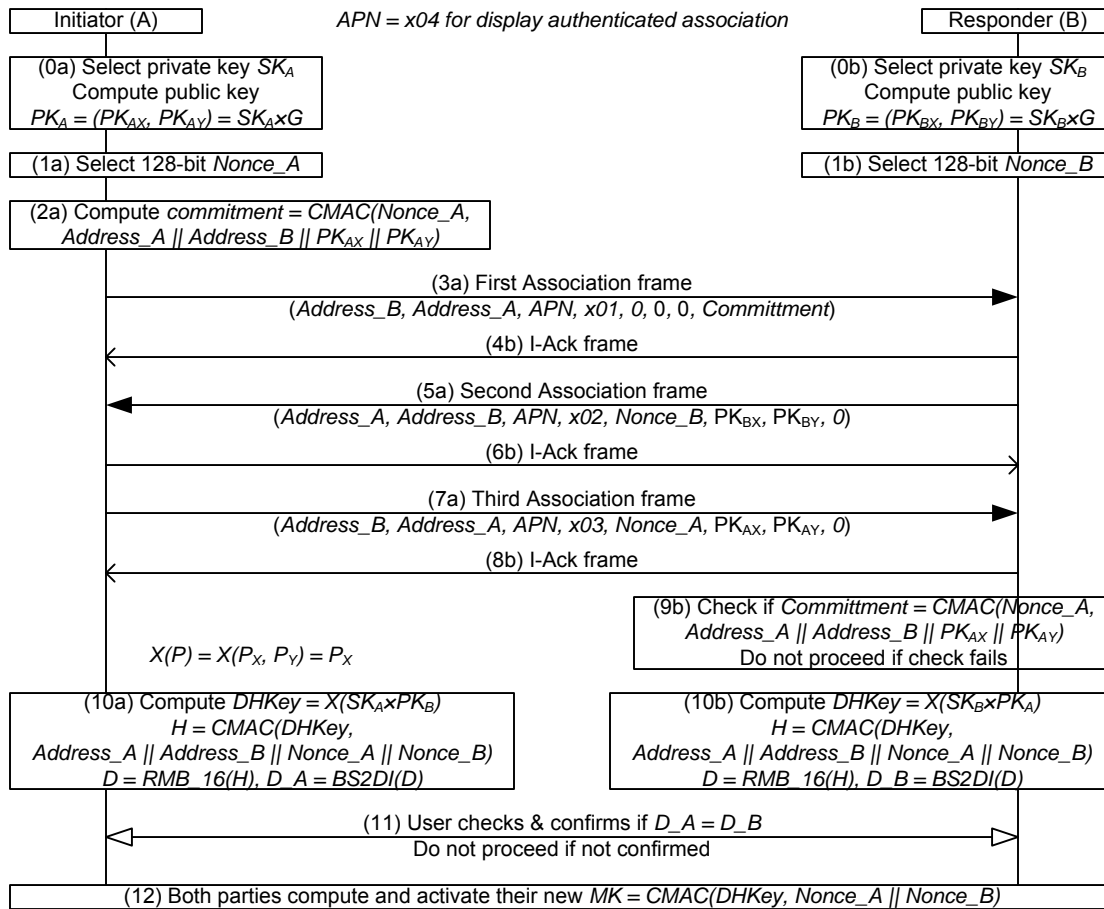
Figure 66 — Display authenticated association procedure
