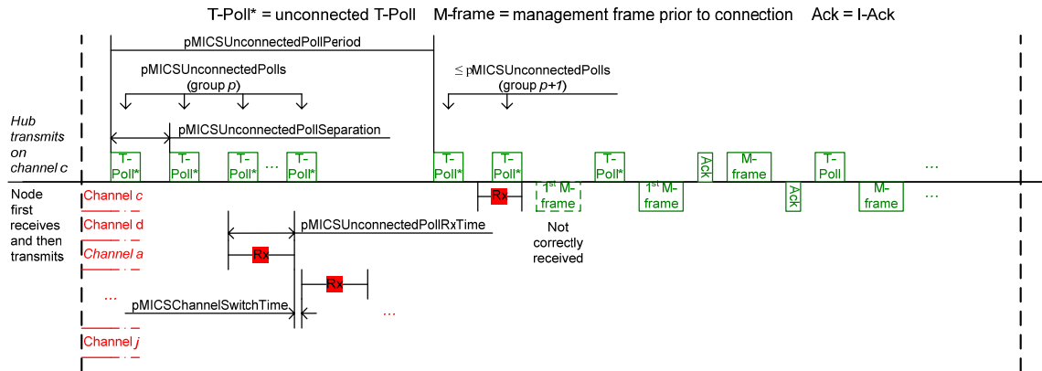
Figure 46 — Unconnected exchange in the MICS band
