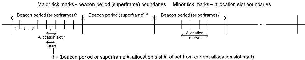
Figure 3 — Time reference base
