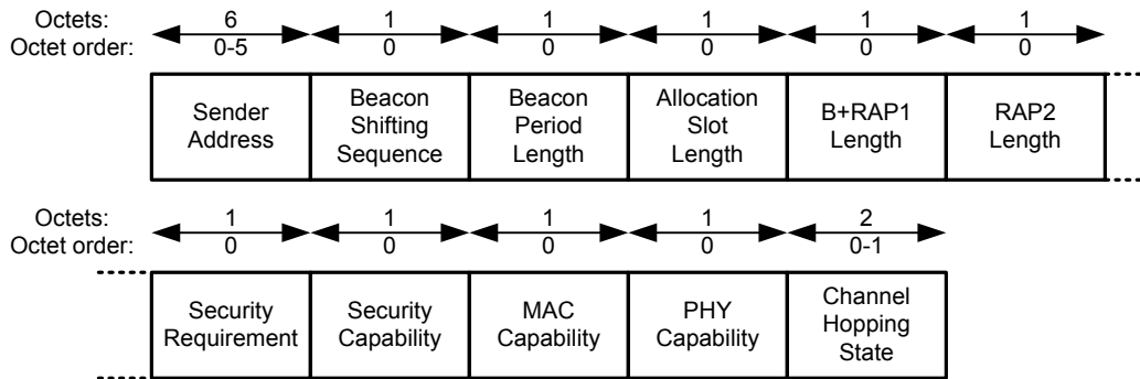
Figure 13 — Frame Payload format for beacon frames
