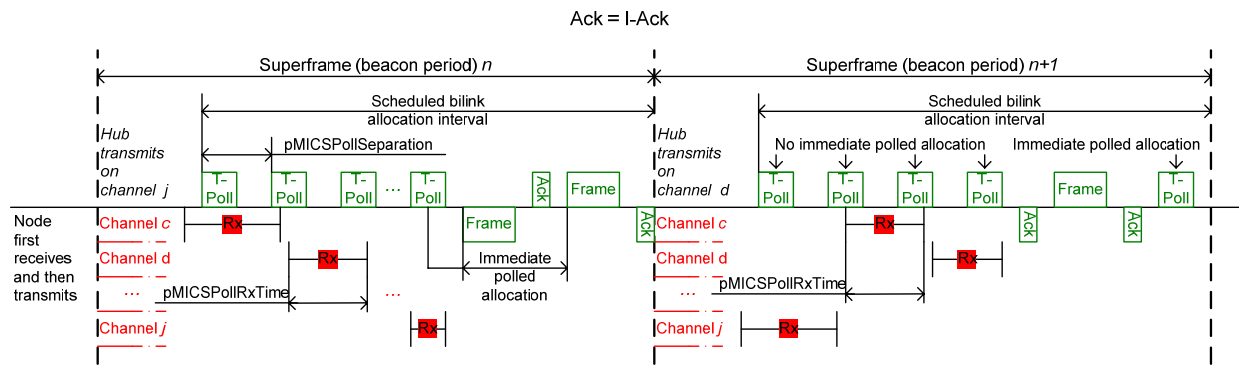
Figure 47 — Connected exchange in the MICS band
