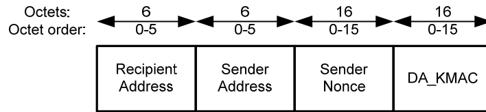
Figure 22 — Frame Payload format for Disassociation frames
