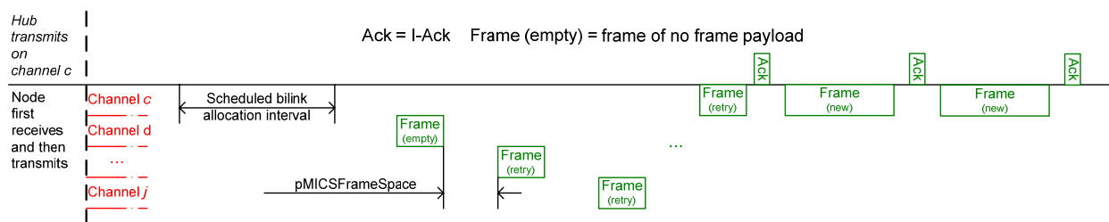
Figure 48 — Medical implant event report outside scheduled allocation intervals in the MICS band
