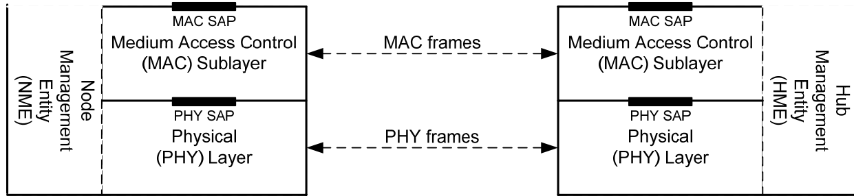
Figure 2 — Reference model
