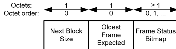
Figure 29 — Frame Payload format for B-Ack frames
