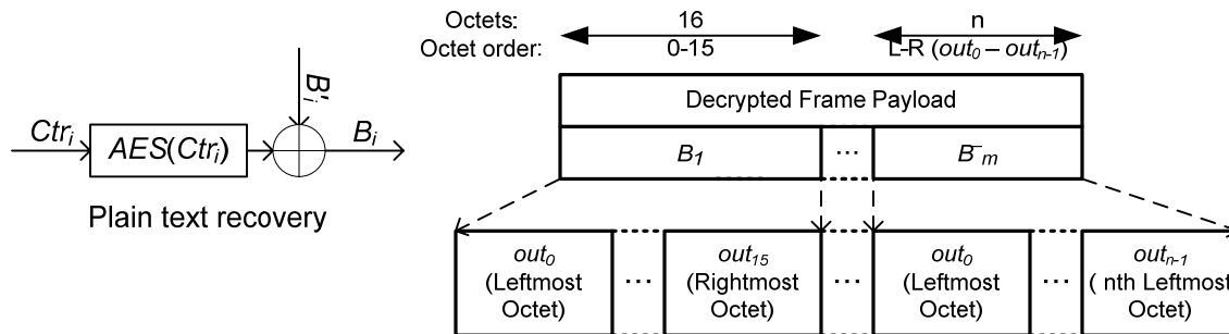
Figure 61 — Decrypted Frame Payload format for encrypted frames
