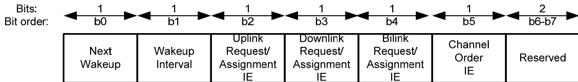
Figure 26 — Change Indication format
