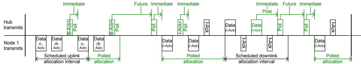
Figure 41 — Example polls and polled allocations
