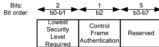
Figure 16 — Security Requirement Format
