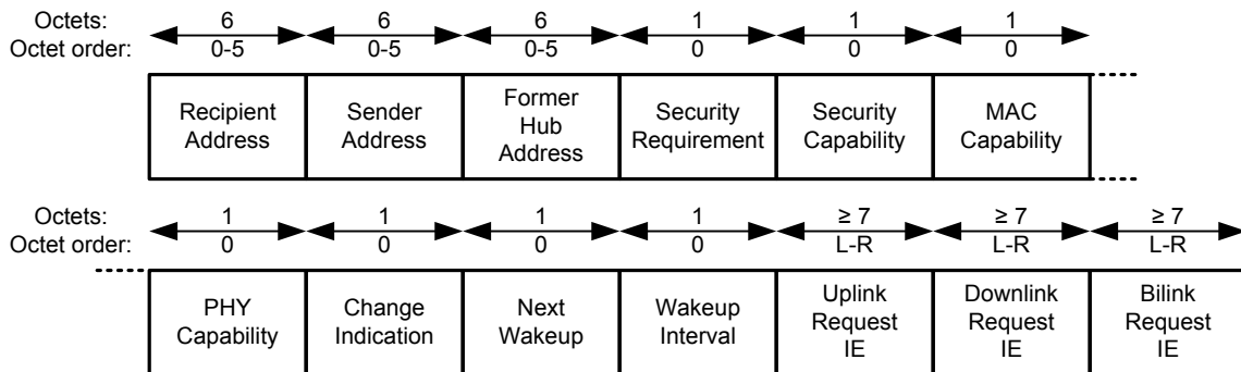
Figure 25 — Frame Payload format for Connection Request frames
