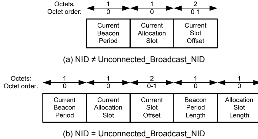
Figure 30 — Frame Payload format for T-Poll frames
