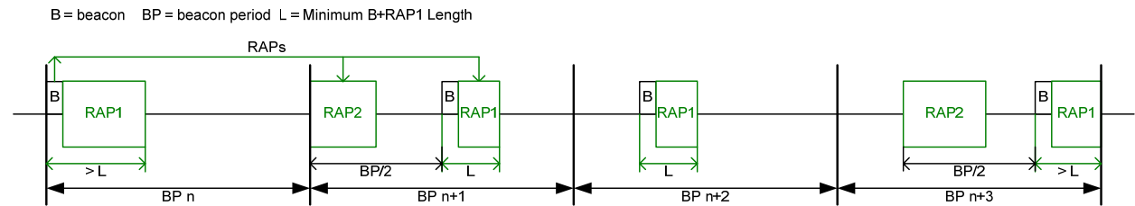
Figure 43 — Random access phases (RAPs)
