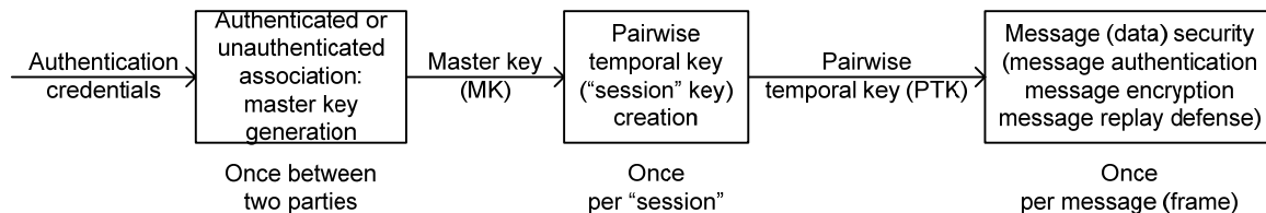
Figure 5 — Security hierarchy
