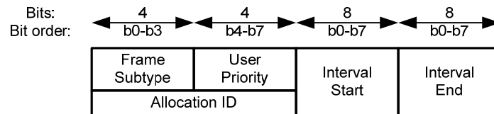
Figure 35 — Allocation Assignment format
