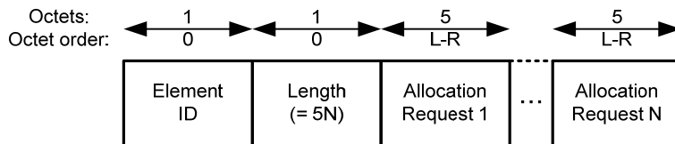
Figure 32 — Uplink Request, Downlink Request, or Bilink Request IE format
