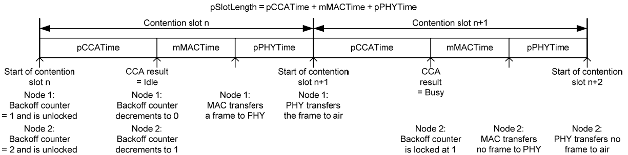
Figure 44 — Contention slot structure
