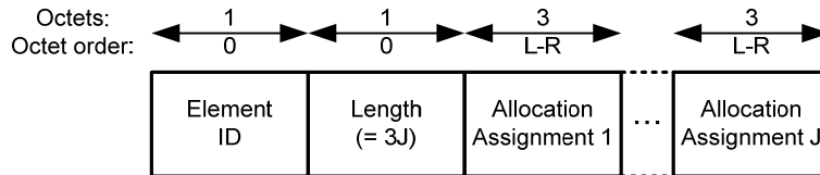
Figure 34 — Uplink Assignment, Downlink Assignment, or Bilink Assignment IE format
