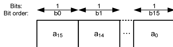
Figure 12 — FCS format
