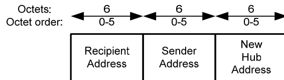
Figure 28 — Frame Payload format for Disconnection frames
