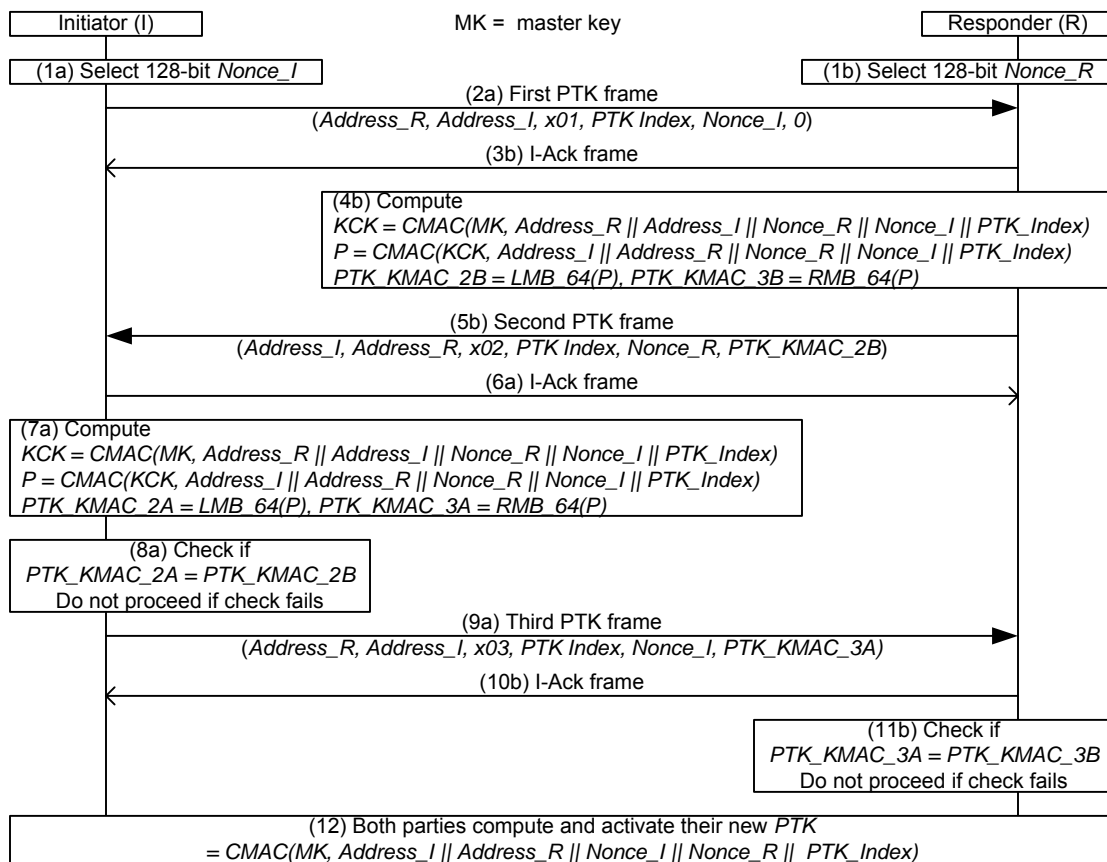
Figure 62 — PTK creation procedure
