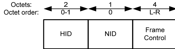
Figure 9 — MAC header format
