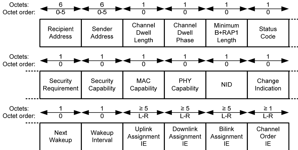
Figure 27 — Frame Payload format for Connection Assignment frames
