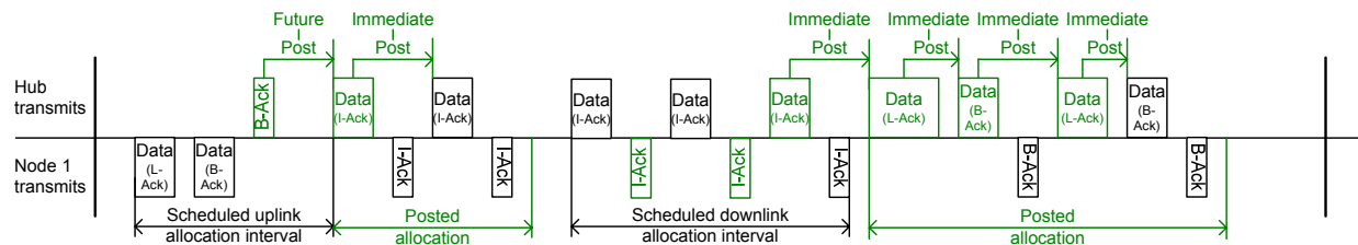
Figure 42 — Example posts and posted allocations
