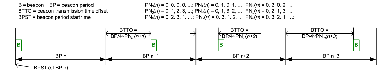
Figure 38 — Beacon transmission
