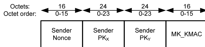
Figure 21 — Association Data format for association protocols 1-4
