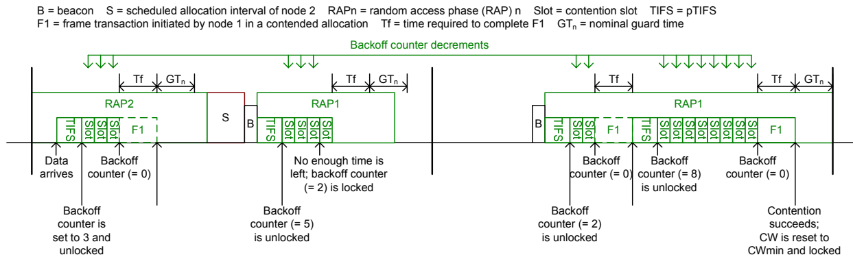
Figure 45 — Example random access
