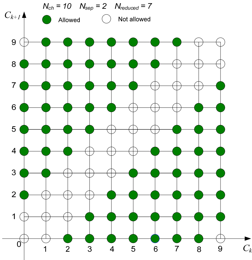
Figure 53 — Channel separation in consecutive hops
