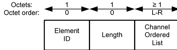
Figure 36 — Channel Order IE format
