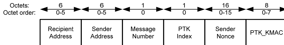
Figure 23 — Frame Payload format for PTK frames
