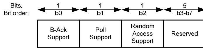
Figure 18 — MAC Capability format
