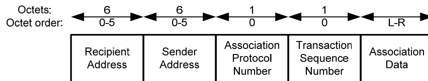
Figure 20 — Frame Payload format for Association frames
