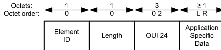
Figure 37 — Application Specific IE format
