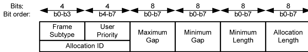
Figure 33 — Allocation Request format
