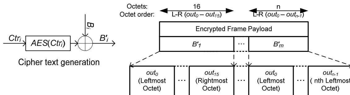
Figure 60 — Encrypted Frame Payload format for encrypted frames
