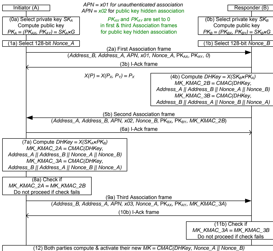
Figure 64 — Unauthenticated association procedure
