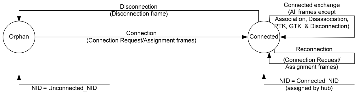
(b) Unsecured communication
