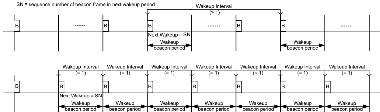
Figure 50 — Macroscopic power management
