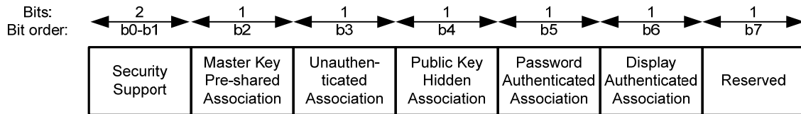
Figure 17 — Security Capability format
