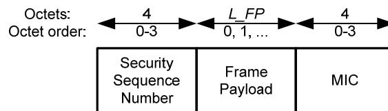
Figure 11 — MAC frame body format
