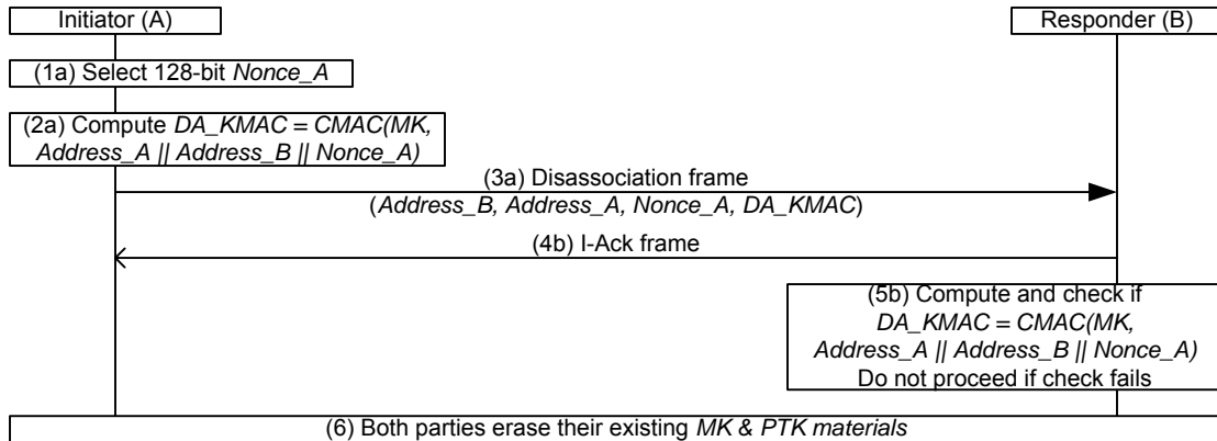
Figure 67 — Disassociation procedure
