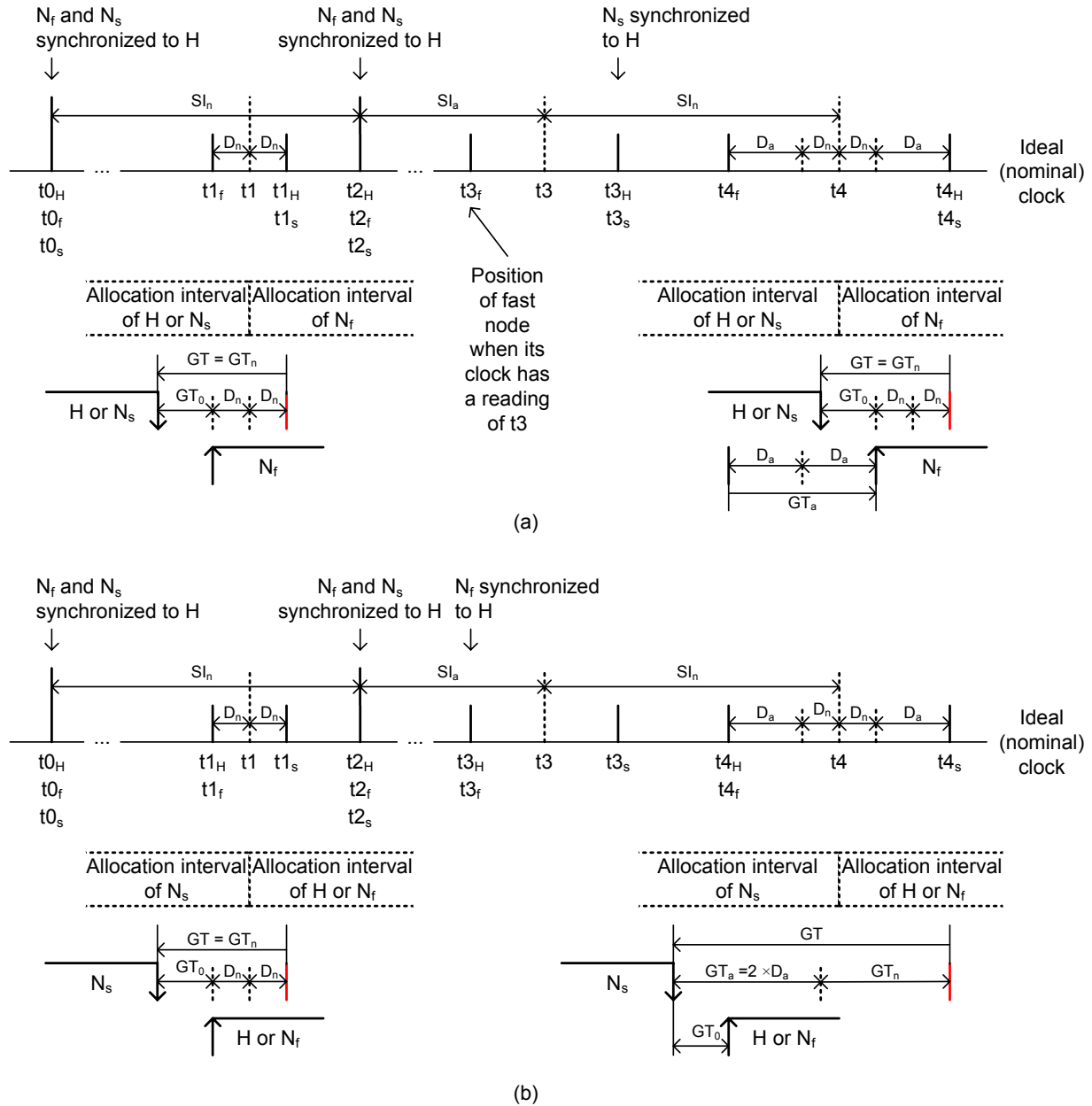
Figure 49 — Clock drifts and guardtimes
