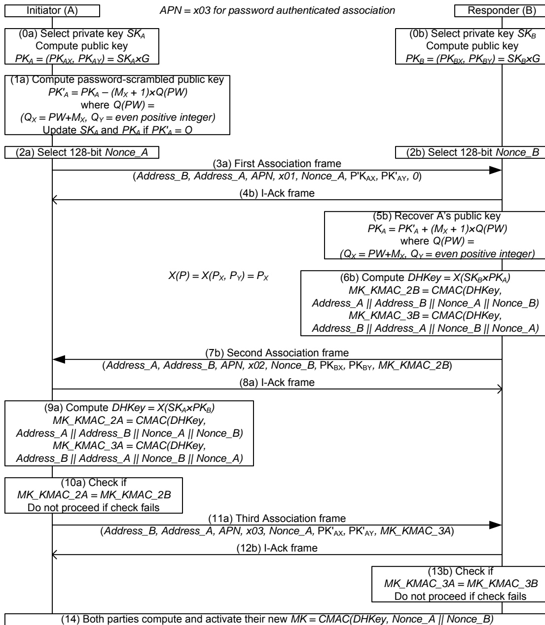
Figure 65 — Password authenticated association procedure
