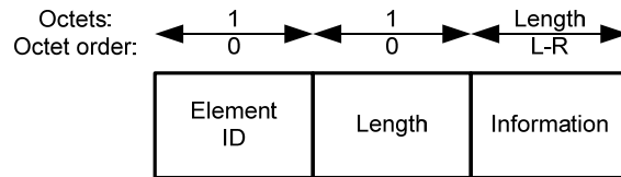
Figure 31 — IE format – general
