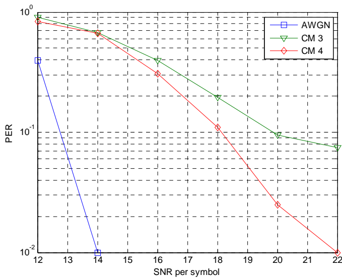
Figure 10.1: PER results for mod-type 3 modulation scheme
