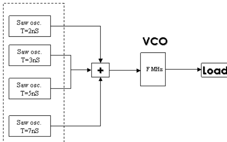
Figure 6.2: Chaos generator using saw tooth pulses.
