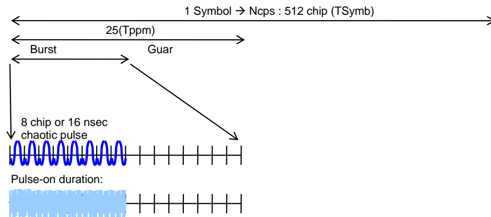
Figure 5.1: symbol structure for 1 Mbps data rate
