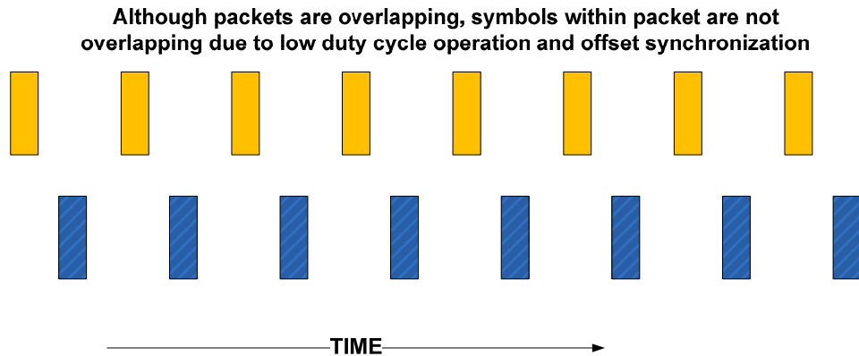
Figure 8.5: Offset piconet synchronization for co-existence with overlapping packets
