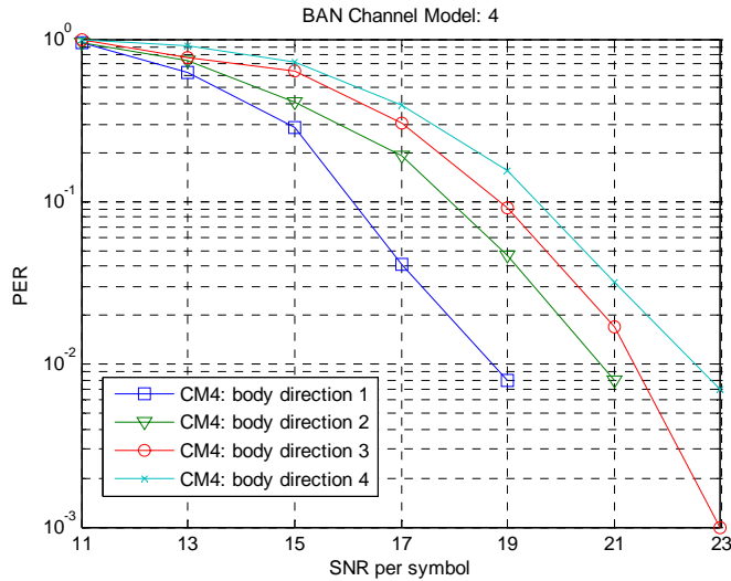
Figure 10.4: PER results for modulation type 0,1,2 modulation schemes for CM4.
