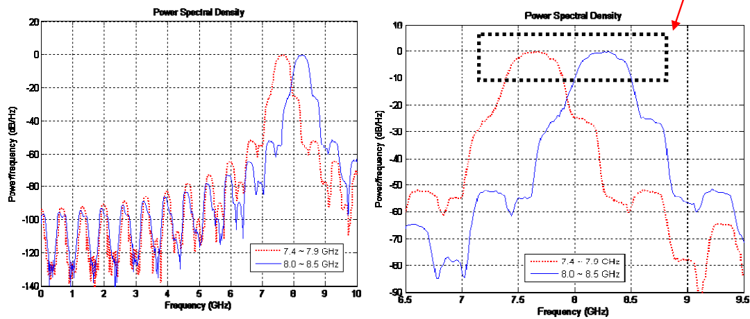
Figure 6.3.: Spectrum of the Chaos Pulses
