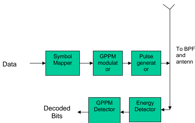
Figure.4. 1 : Block Diagram
