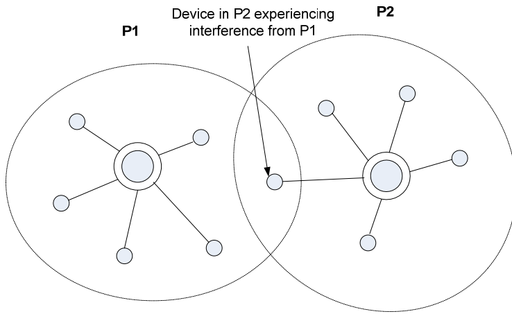
Figure 8.2: Piconet interference between piconets P1 and P2
