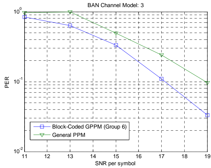
Figure 10.3: PER results for modulation type 0,1,2 modulation schemes for CM3.
