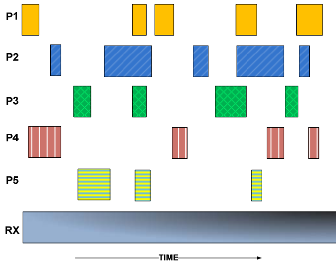
Figure 8.4: Piconet co-existence
