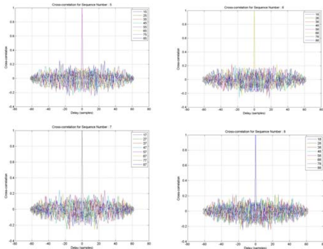
Figure 8.7 : Auto- and cross- correlation properties
