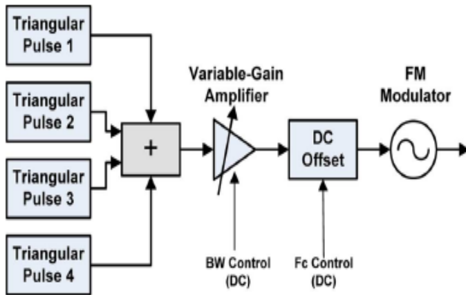
Figure 6.1. Chaos Generator using triangular waveform
