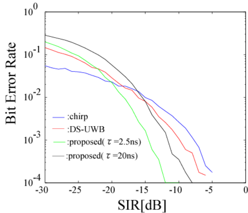
Case of the number of coexisting nodes or BANS is 8 (Bit rate = 1Mbps)
