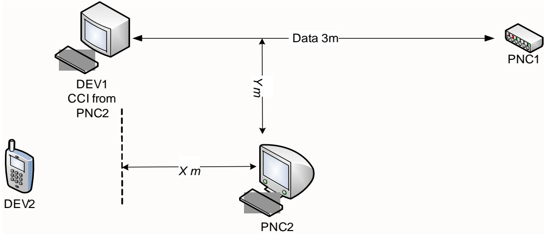
Figure 8—Relative position of devices for coexistence scenario 2.
