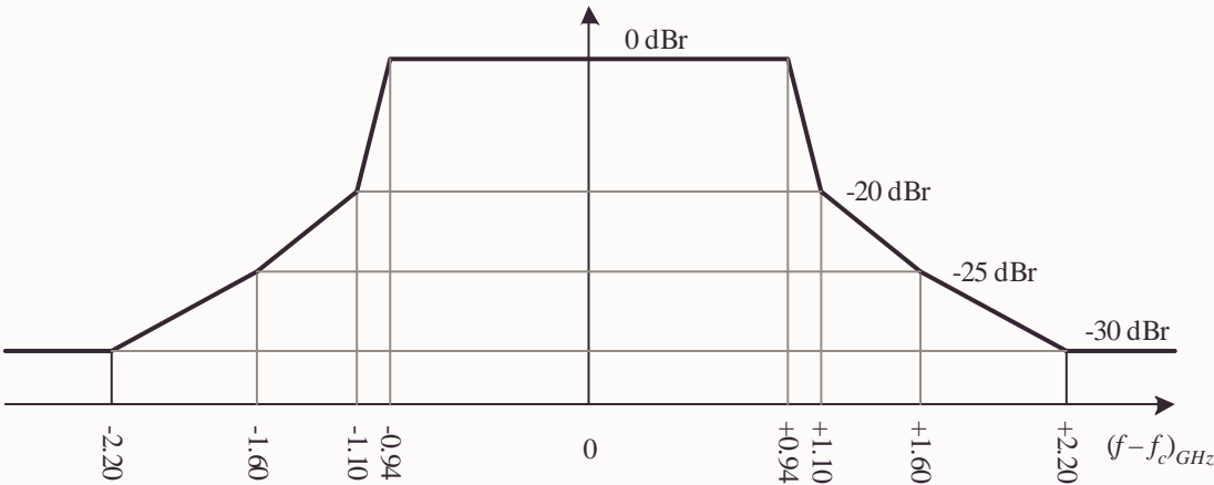
Figure 1—Transmit spectral mask
