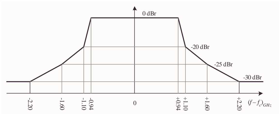
Figure 2—Transmit spectral mask
