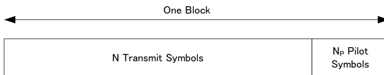
Figure D3.1 - Formation of Pilot Insertion
