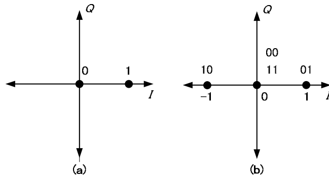
Figure 189 Constellation Diagram for (a) OOK and (b) DAMI
