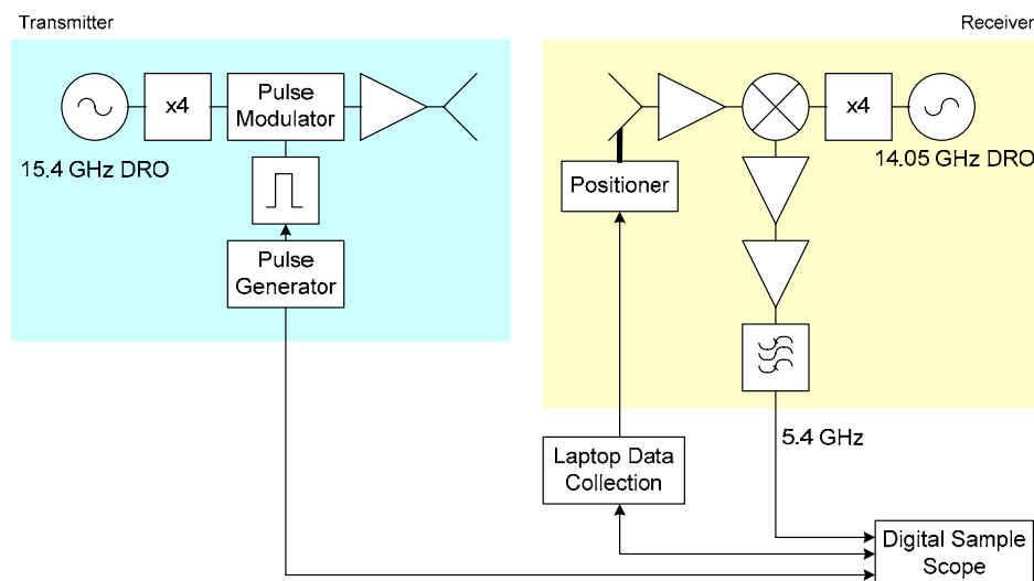
Figure 1. Measurement setup
