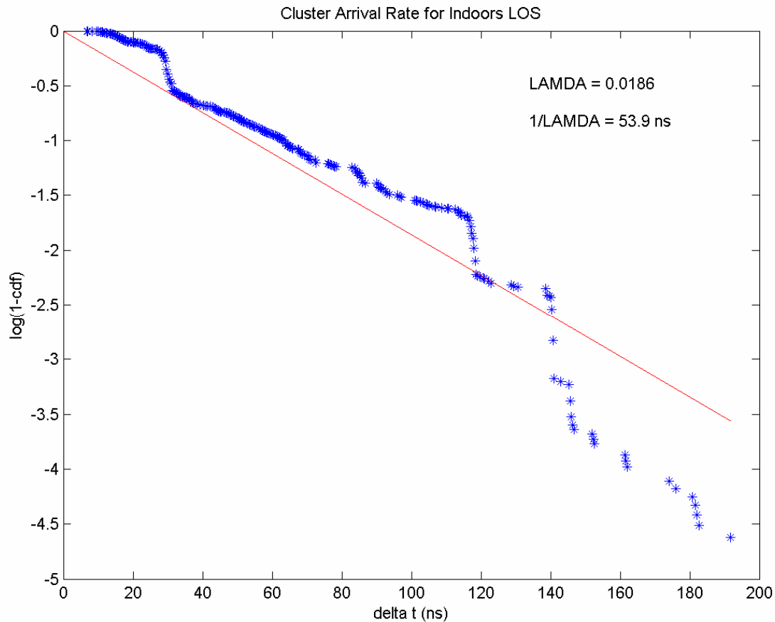
Fig. (14): \Lambda = 0.0186 for OFF_LOS
