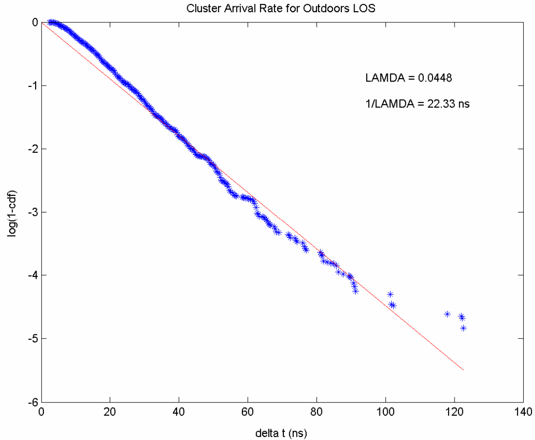
Fig. (17): \Lambda = 0.0448 for OUT_LOS
