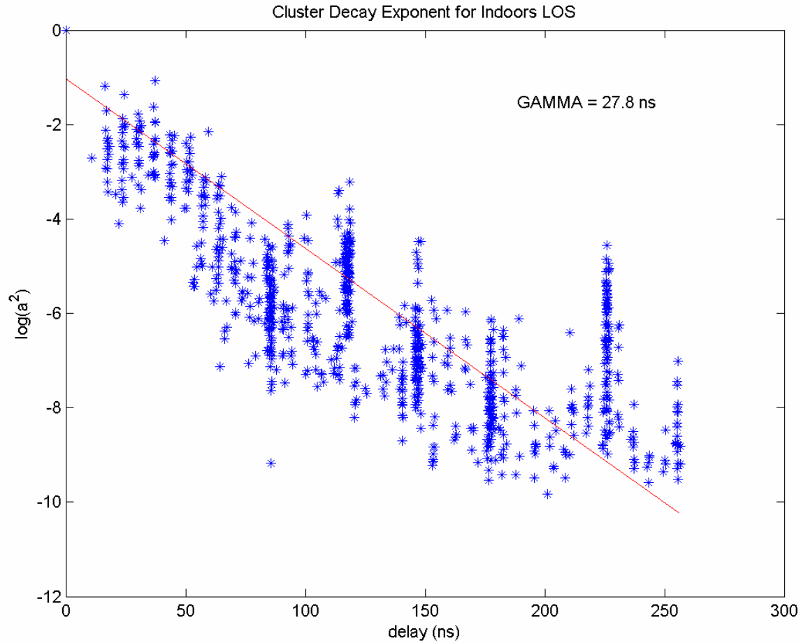
Fig. (6): \Gamma = 27.8 for OFF_LOS
