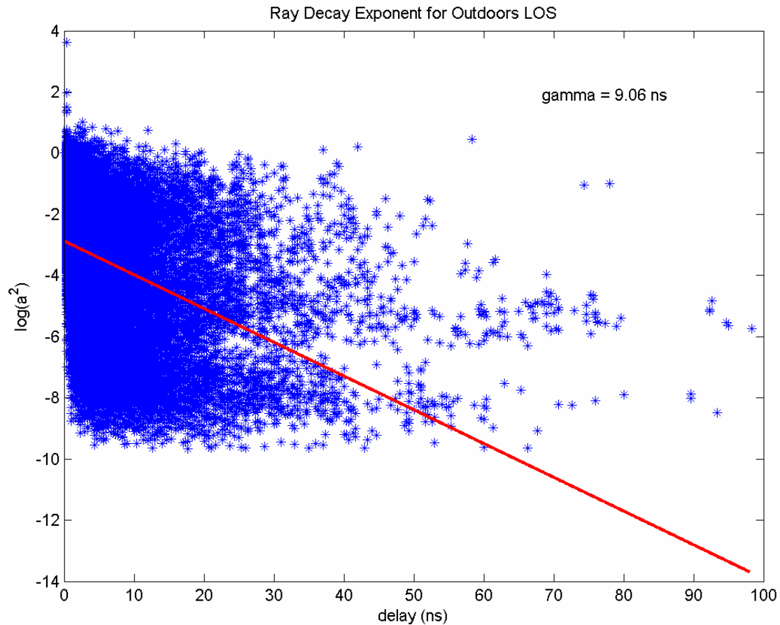
Fig. (1): \gamma = 9.1 for OUT_LOS
