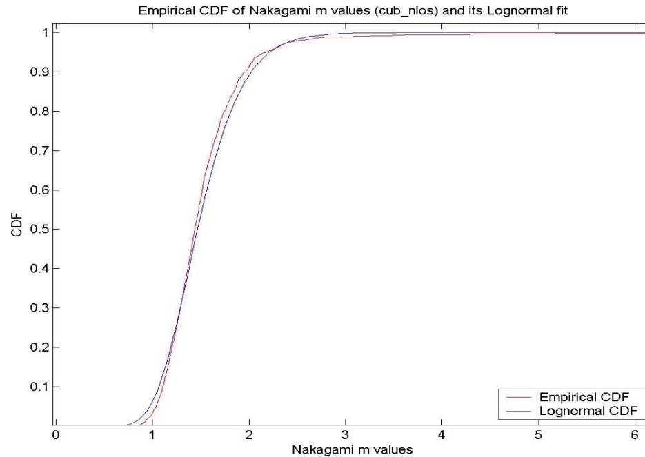
Fig. (28): cdf of 'm' OFF_SOFT_NLOS : \mu_m = 0.38 , \sigma_m = 0.25
