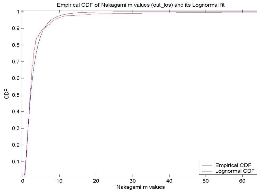
Fig. (29): cdf of 'm' OUT_LOS: \mu_m = 0.78 , \sigma_m = 0.78
