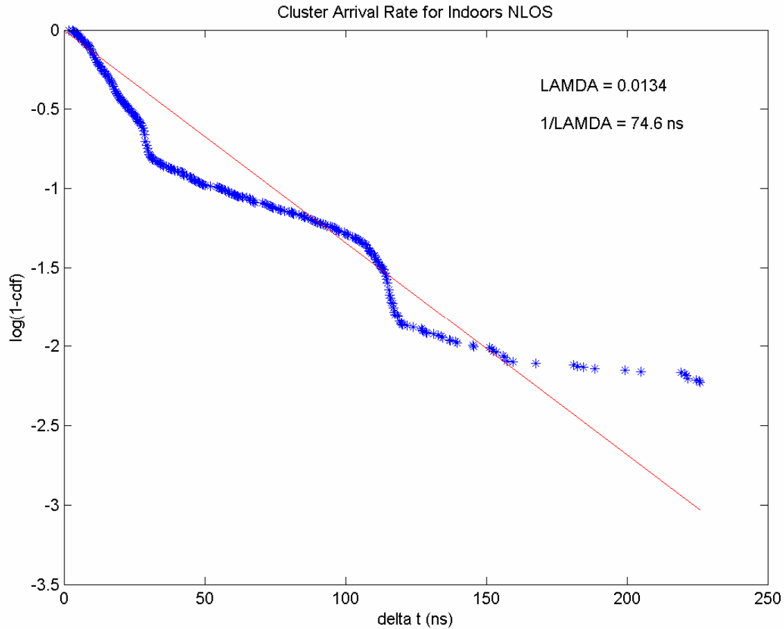
Fig. (15): \Lambda = 0.0134 for OFF_SOFT_NLOS
