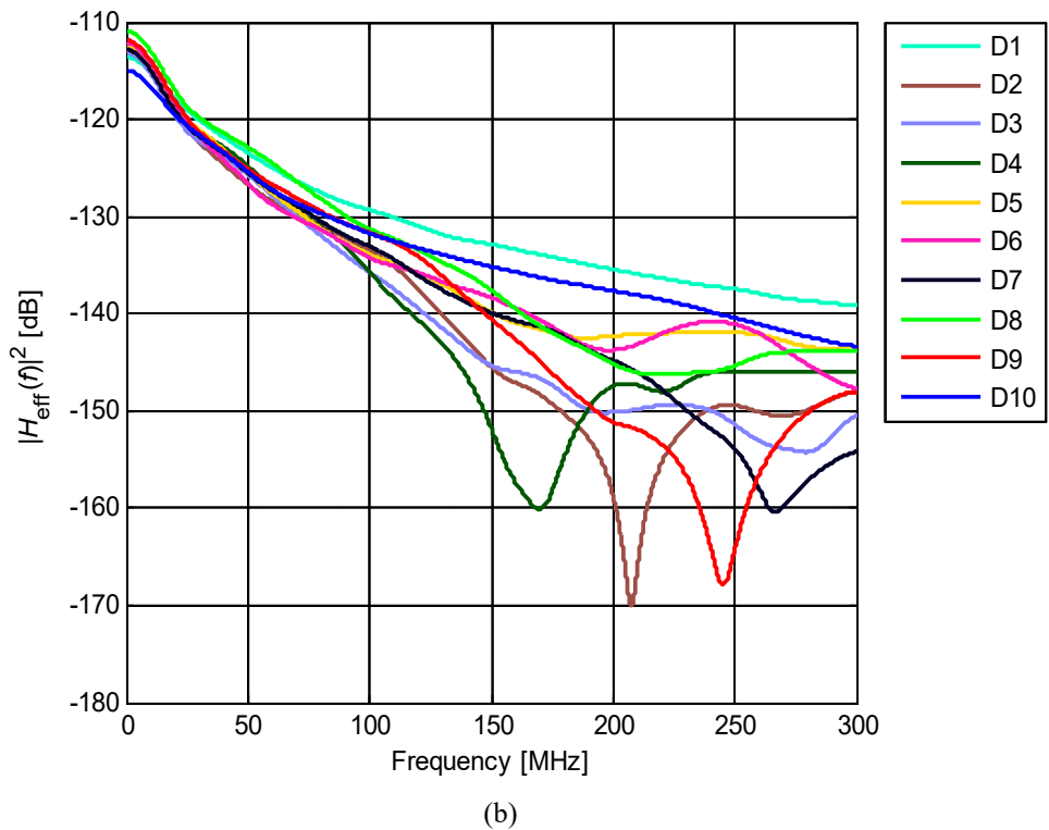
Fig. 15. (a) Optical channel responses and (b) effective channel responses for conference room
