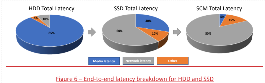
Figure 6 – End-to-end latency breakdown for HDD and SSD
