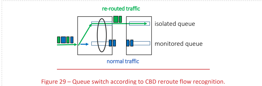
Figure 29 – Queue switch according to CBD reroute flow recognition.
