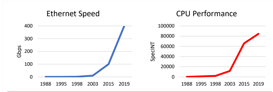
Figure 10 – Historical Performance Comparison
