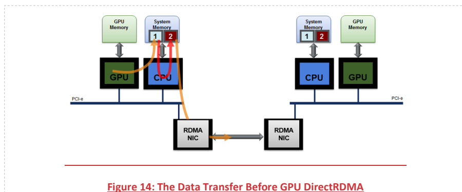
Figure 14: The Data Transfer Before GPU DirectRDMA
