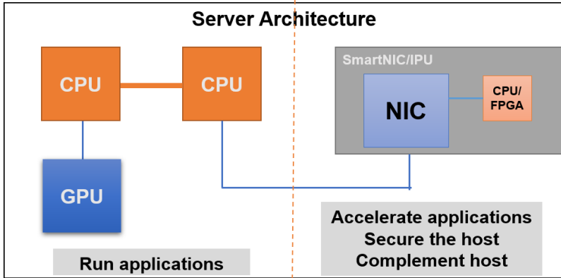
Figure 11 – Server Architecture with SmartNIC
