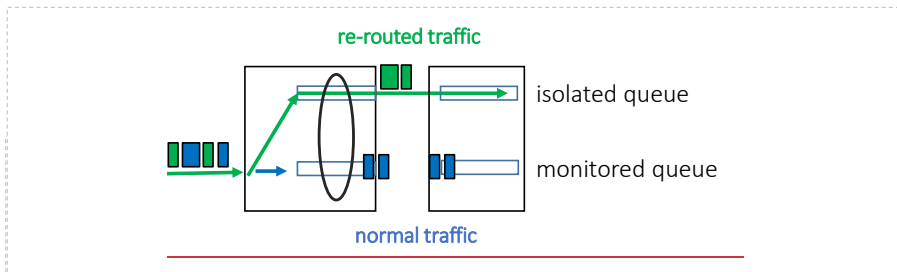
Figure 26 – Queue switch according to CBD reroute flow recognition
