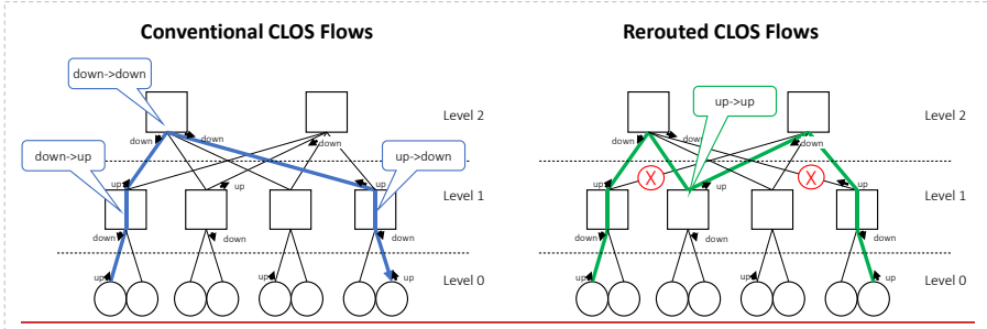
Figure 26 – Identifying CBD points in rerouted flows
