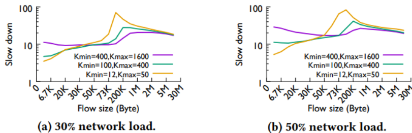
Figure 14 – FCT slowdown distribution with different ECN thresholds, using WebSearch
