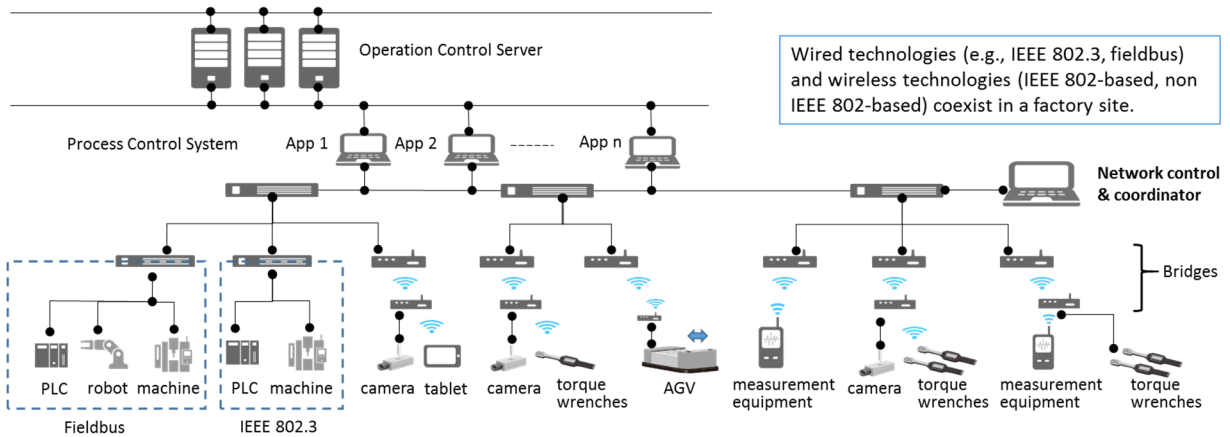
Figure 2—Example of network topology for a vehicle assembly line
