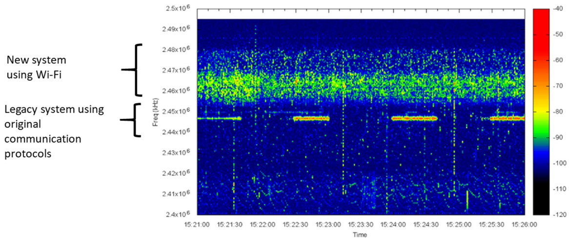
Figure 6—Wireless signals with coexistence of different wireless technologies—The vertical and horizontal-axes show frequency (Hz) and time, and color shows signal strength (dBm) in a bar on the right hand side
