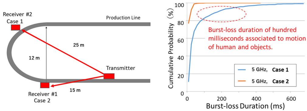
Figure 16—Burst-loss measurement in a large machine assembly site [26]
