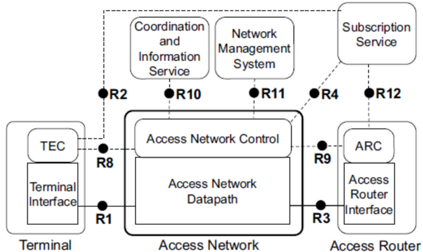
Figure 20—Network reference model defined in IEEE Std 802.1CF
