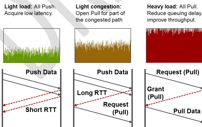
Figure 14 – Push and Pull Hybrid Scheduling
