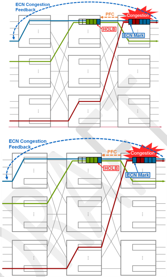
Figure 10 – PFC Head-of-Line Blocking
