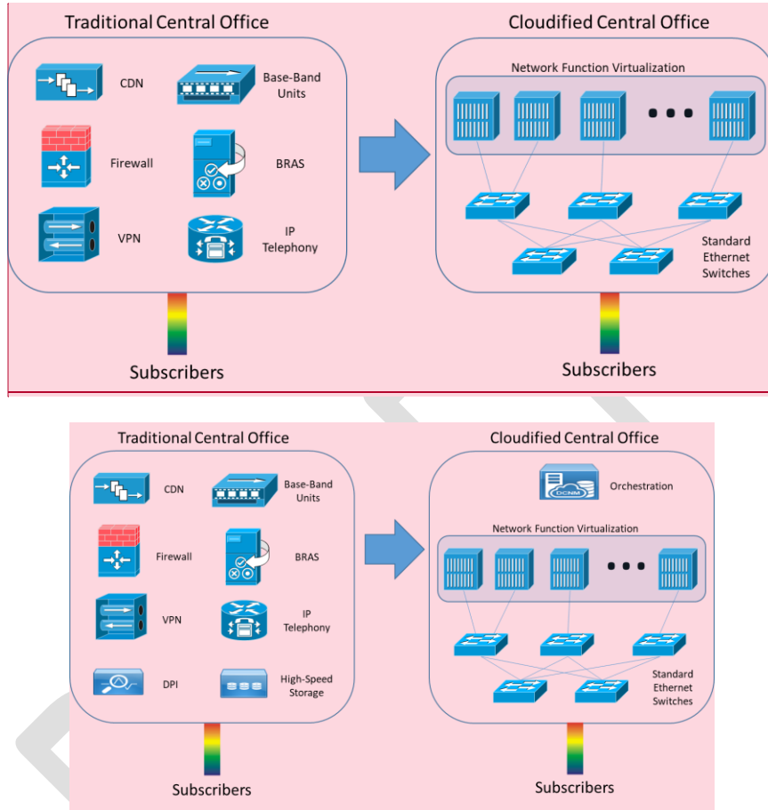
Figure 4 – Transition to Cloudified Architecture in the CO
