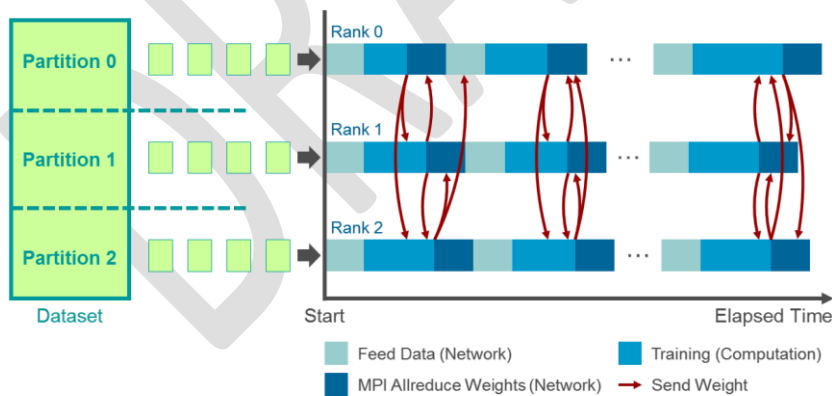
Figure 2 – Deep Learning Training
