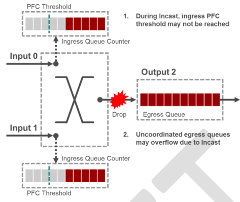
Figure 11 – Switch Packet Loss
