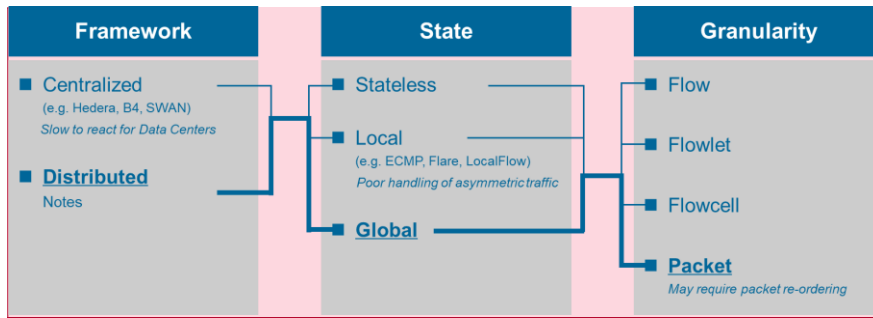
Figure 13 – Load Balancing Design Space
