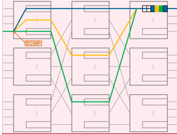
Figure 7 – ECMP Load Balancing
