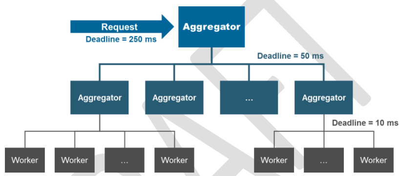
Figure 1 – Parallel Application Hierarchy
