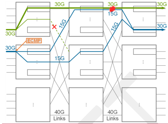
Figure 9 – ECMP Load Balancing Collisions
