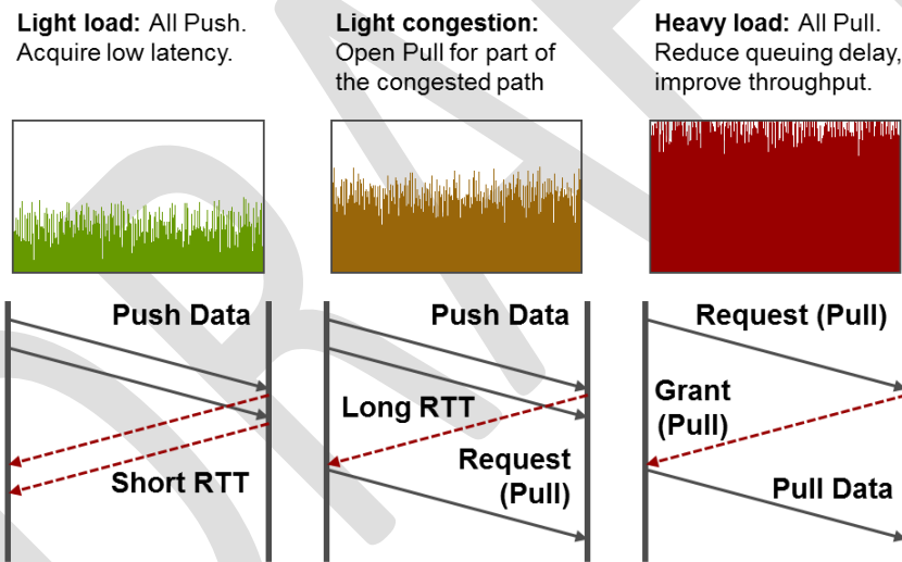
42 43 44 45 46 47 48 49 50 51 52 53 54 Figure 14 – Push and Pull Hybrid
