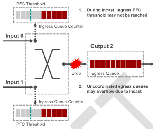
Figure 11 – Switch Packet Loss
