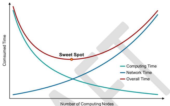
Figure 3 – Parallelism Tradeoff
