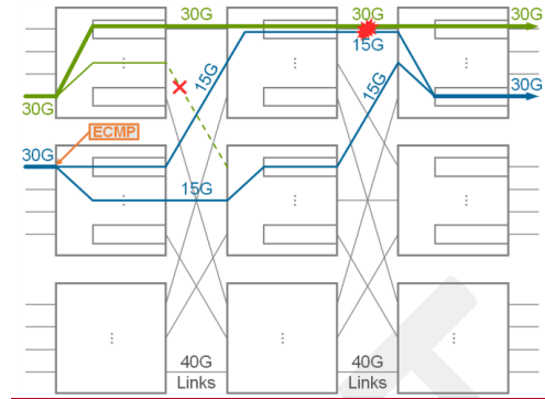
Figure 9 – ECMP Load Balancing Collisions
