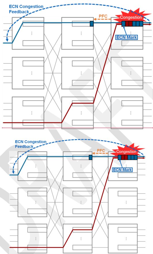
Figure 8 – Current Congestion Management
