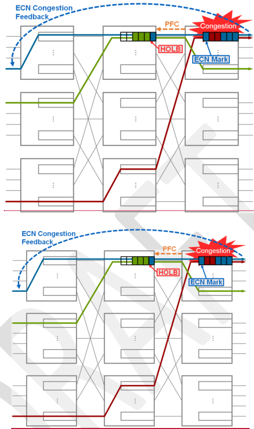
Figure 10 – PFC Head-of-Line Blocking
