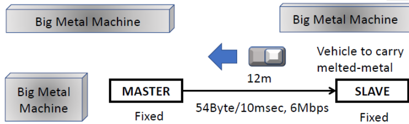
8 Figure 3 Layout in factory for which measurement of RSSI is recorded
