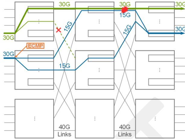
Figure 9 – ECMP Load Balancing Collisions
