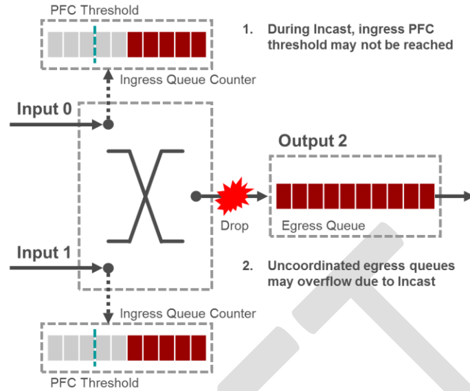
Figure 11 – Switch Packet Loss
