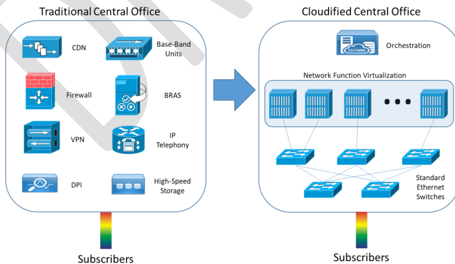
Figure 4 – Transition to Cloudified Architecture in the CO
