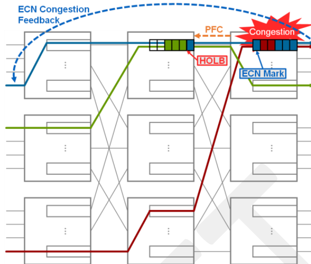
Figure 10 – PFC Head-of-Line Blocking
