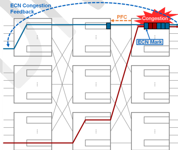
Figure 8 – Current Congestion Management
