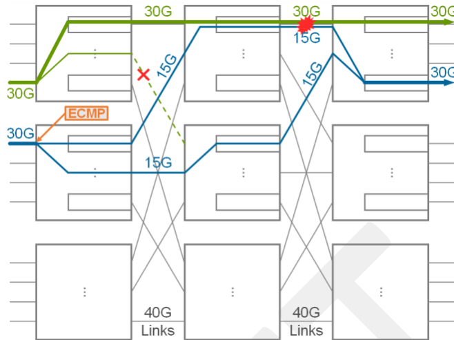
Figure 9 – ECMP Load Balancing Collisions
