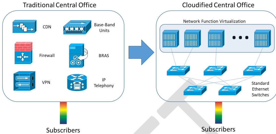
Figure 4 – Transition to Cloudified Architecture in the CO
