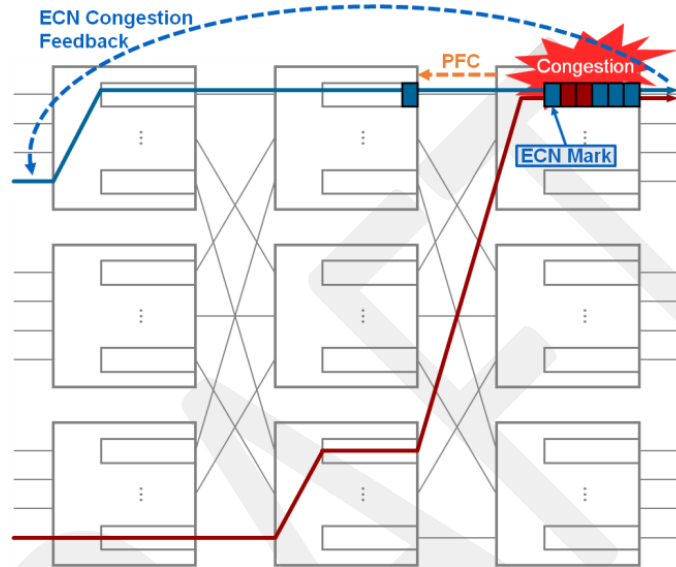
Figure 8 – Current Congestion Management
