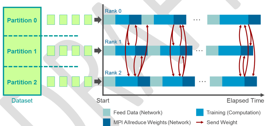
Figure 2 – Deep Learning Training
