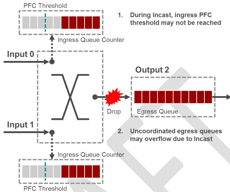
Figure 11 – Switch Packet Loss
