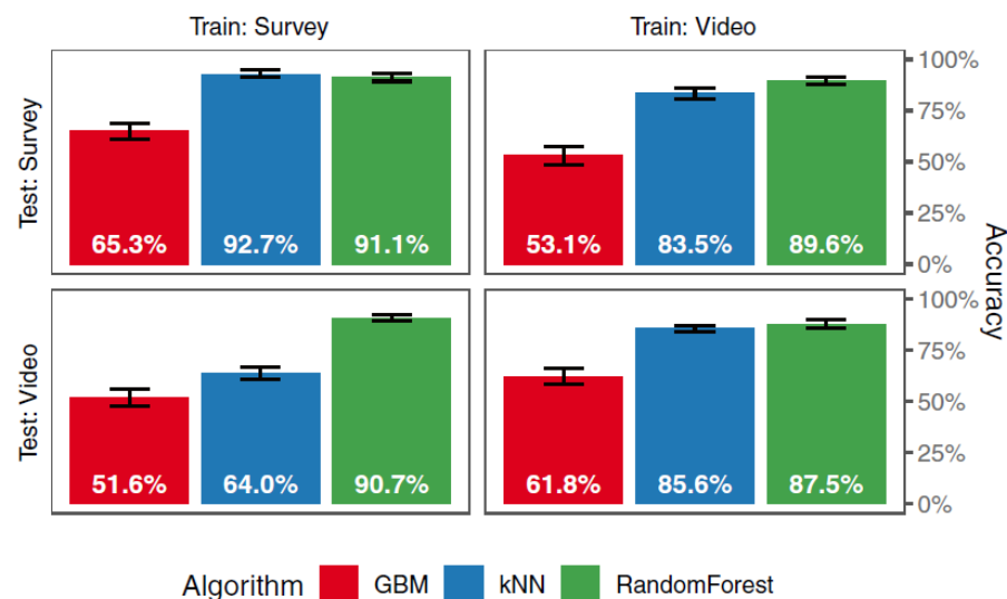
Figure 4. Accuracy within and between tasks. Error bars show the range of all 20 Monte-Carlo cross-validations.
