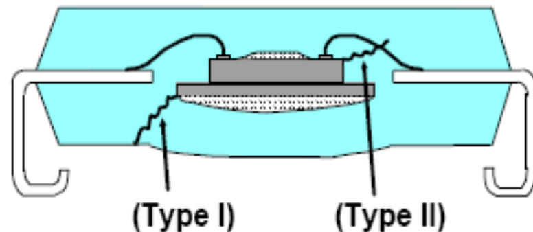
“POPCORN” CRACKS
