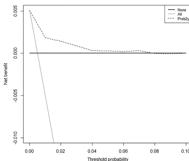
Figure 1 Decision curve for a model to predict liver disease diagnosis in patients having their liver function tests (LFTs) measured in primary care. Dashed line: prediction model; grey line: assume all patients have liver disease; black line: assume no patients have liver disease.
