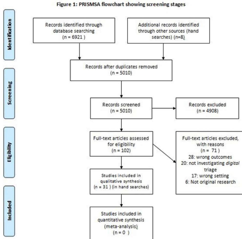
Figure 1: PRISMA Flowchart
