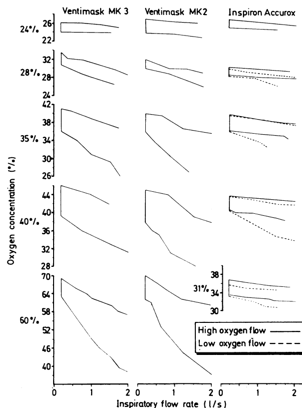
FIG 2—Inspired oxygen concentrations at various inspiratory flow rates (envelope diagrams showing data obtained in all subjects).
