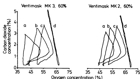
FIG 3—Gas R lines at varying peak inspiratory flow rates: a=1.2 l/s, b=0.8 l/s, c=0.4 l/s, d=0.2 l/s.
