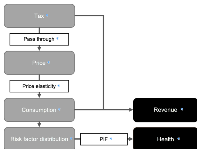
Figure 1 Model structure.
