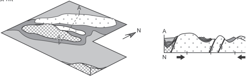
7c. Late Syn-rift
