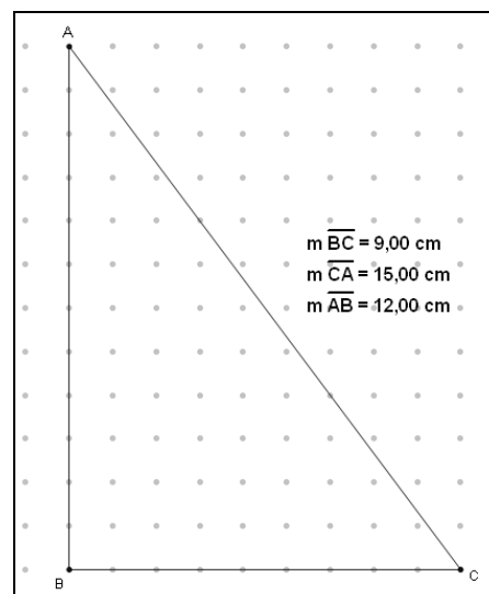
Figure 3. Investigating Pythagorean triples in a dynamic geometry application
