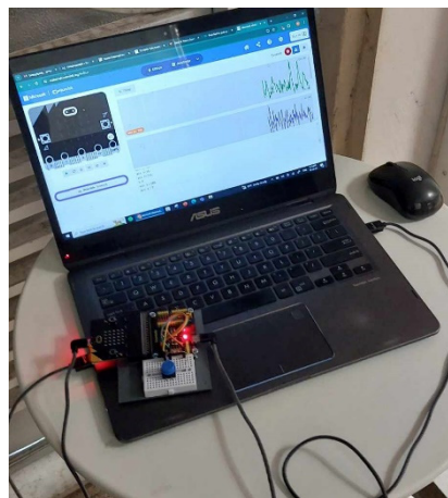
Figure 15. Receiver System
