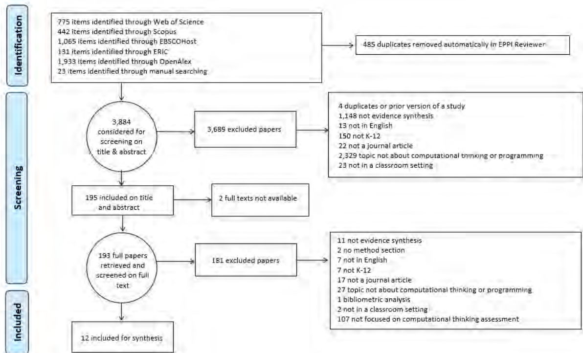
Figure 2. PRISMA diagram
