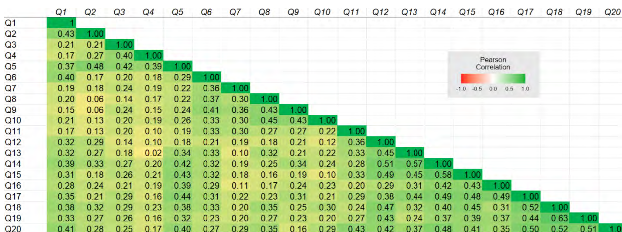
Figure 1. Correlation Heatmap.
