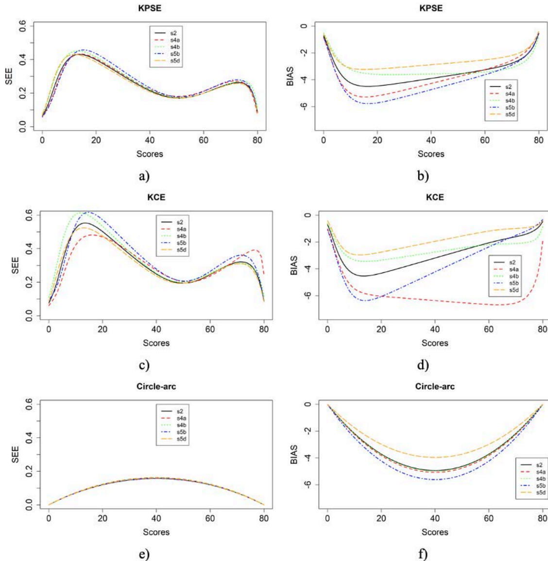
Figure 6. SEE (left) and bias (right) for groups differing in ability and difficulty of the anchor test form was varied (s2, s4a, s4b, s5b and s5d).
