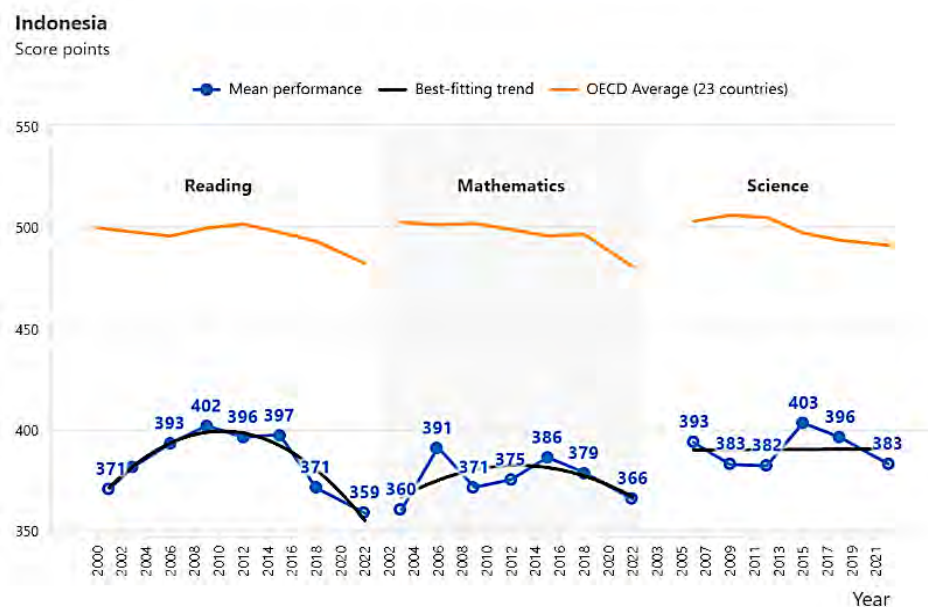
Figure 1: Indonesian Students' Scores in PISA
